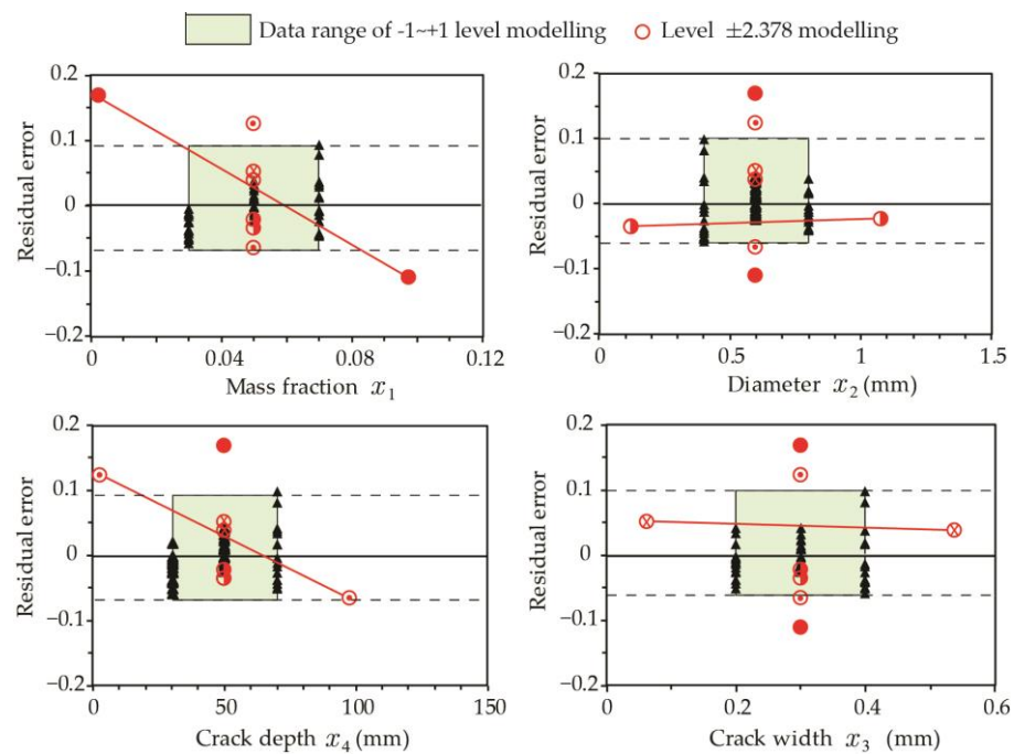
Figure 8. Influence of individual factors on residual errors of model-Ph. The results of extreme cases at Level ±2.378 are connected by a red line.
