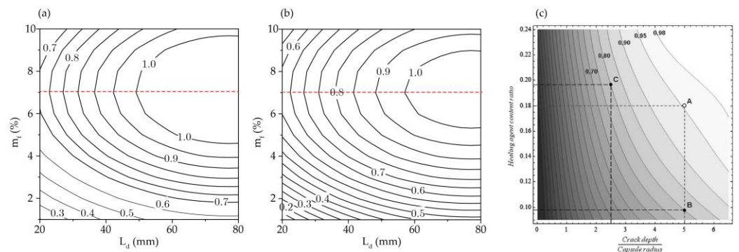
Figure 16. Contour plot of hitting probability P_h as a function of L_D and m_f for (a) d = 0.2 mm, L_w = 0.3 mm and (b) d = 0.6 mm, L_w = 0.3 mm; (c) Hitting probability as a function of normalized crack depth and volume fraction of capsules, for a cube of side length equivalent to 1 cm containing 27 capsules, with V_{\text{capsule}}/V_{\text{cube}} varying from 0.1–0.3 [19].
