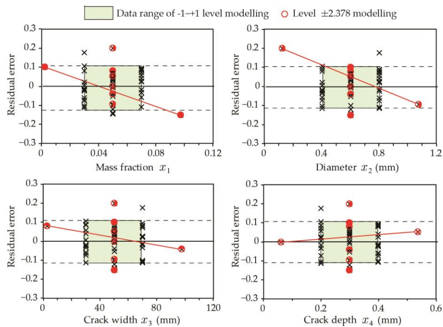
Figure 10. Influence of individual factors on residual errors of model-H 0 . The results of extreme cases at Level ±2.378 are connected by a red line.
