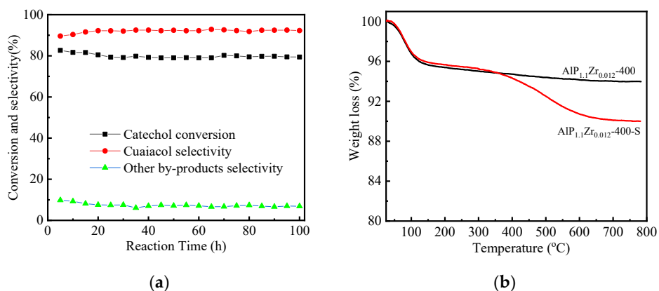
Figure 8. (a) Catalytic properties as a function of time for the selective O -methylation of catechol over AlP 1.1 Zr 0.012 -400 catalysts. Reaction condition: m_{\text{cat}} = 2 g, Reaction temperature = 280 °C, LHSV = 0.2 h -1 , methanol/catechol = 5 (mol). (b) TG profiles of the AlP 1.1 Zr 0.012 -400 and AlP 1.1 Zr 0.012 -400-S catalysts.
