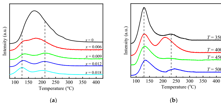
Figure 5. CO 2 -TPD patterns of (a) AIP 1.1 Zr x -400 and (b) AIP 1.1 Zr 0.012 - T samples.
