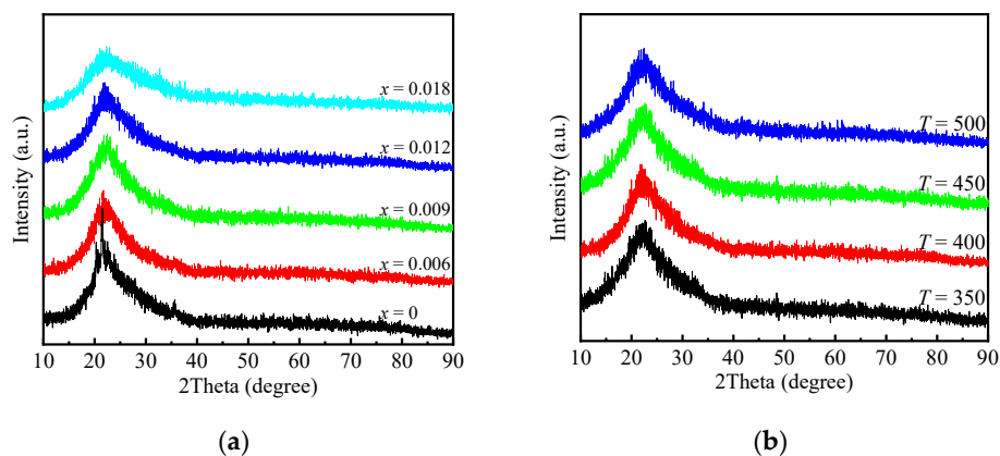
Figure 1. XRD patterns of the (a) AlP_{1.1}Zr_x -400 and (b) AlP_{1.1}Zr_{0.012} - T samples.
