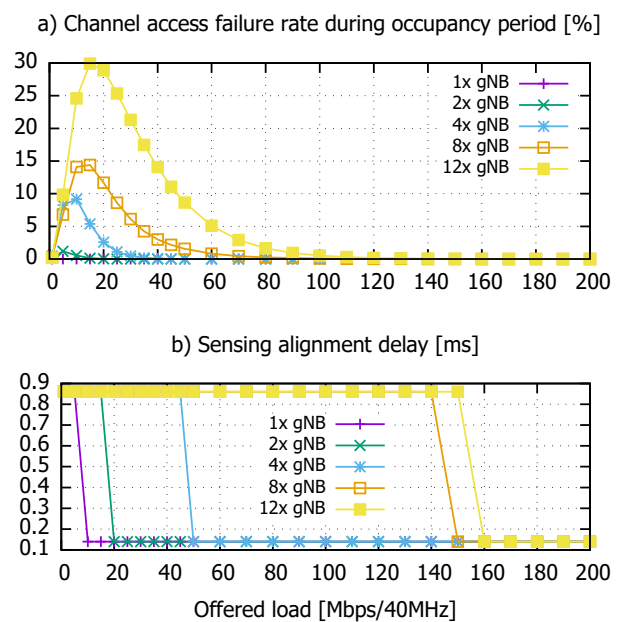
FIGURE 8. NR-U FBE KPI analysis for different network configurations.
