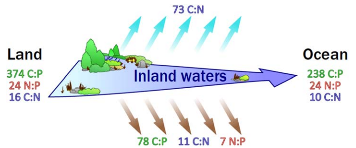
Fig. 3. Global estimates of stoichiometry of the freshwater pipe. C : P, N : P, and C : N molar ratios of estimated inputs from terrestrial systems, loss to burial and the atmosphere and export to the ocean. Figure adapted from Cole et al. (2007, fig. 1).
