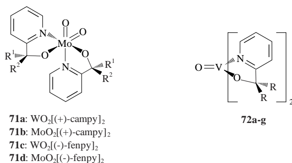
Figure 13. Chiral Mo and achiral V complexes.
