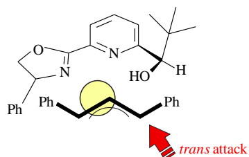
Scheme 20. Nucleophilic allylic attack in Pd-catalysed allylic alkylation in the presence of pyridinooxazoline ligands.
