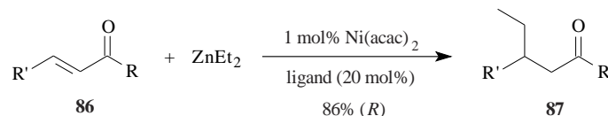
Scheme 8. Nickel-catalysed conjugate addition of Et 2 Zn to chalcones.
