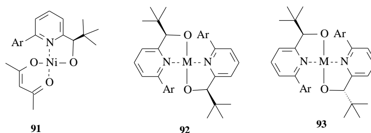
Figure 17. Intermediates proposed for the Ni-catalyzed addition reactions [74,75].
