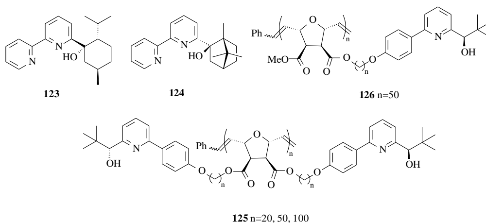
Figure 25. Bipyridyl and polymer-supported pyridyl alcohol ligand precursors.
