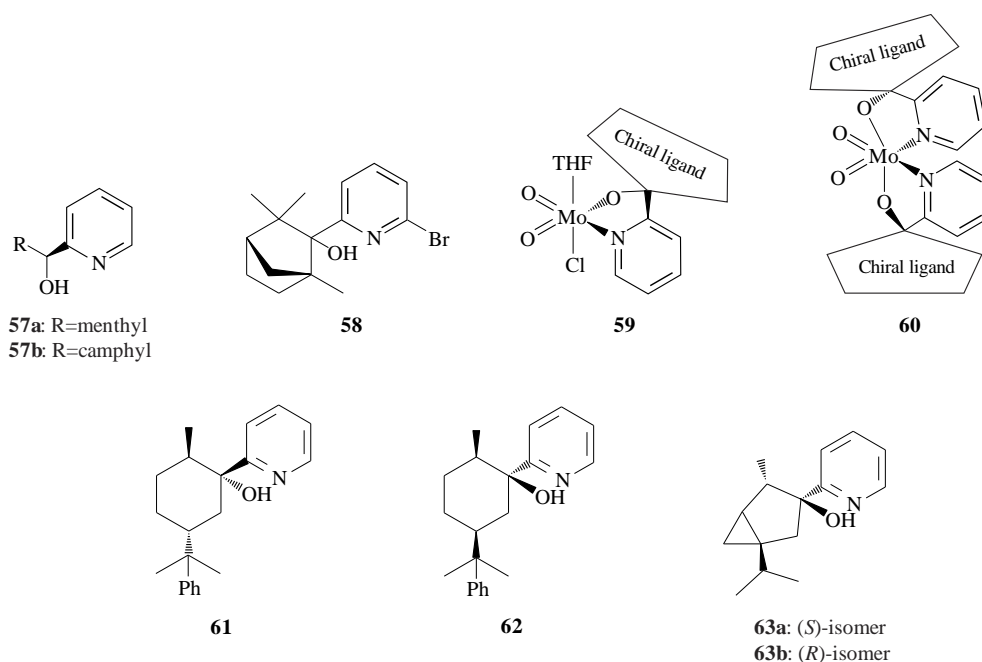
Figure 11. Chiral pyridinyl alcoholato ligands and Mo complexes.
