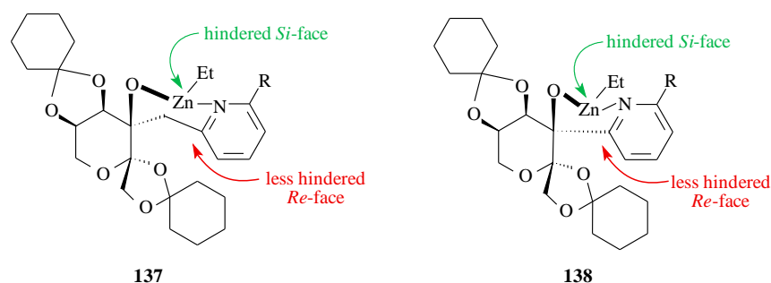
Scheme 11. Mechanism of Et 2 Zn addition to benzaldehyde using pyridinyl alcohols 137 and 138 .
