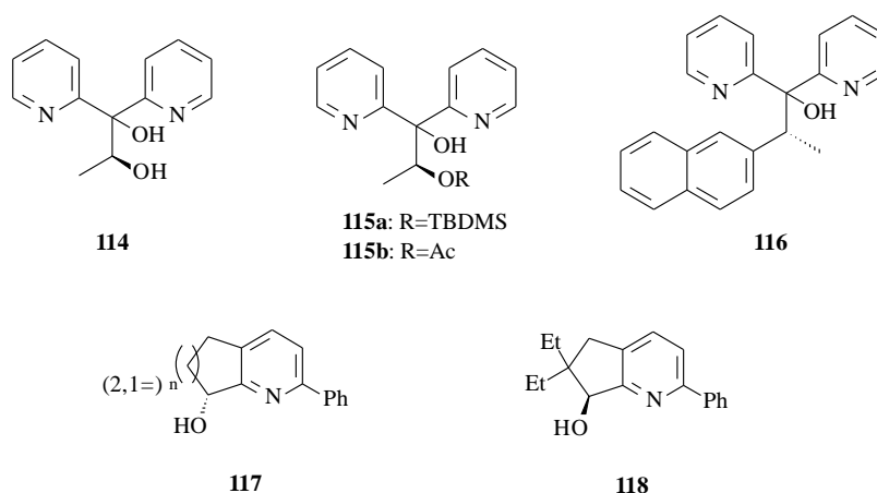
Figure 23. Pyridinyl alcohols used as ligands in the addition of diethylzinc to benzaldehyde.
