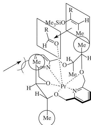
Scheme 18. A model transition state for the aldol reaction of silyl enol ether in \text{Pr}^{3+} - 154 complex.
