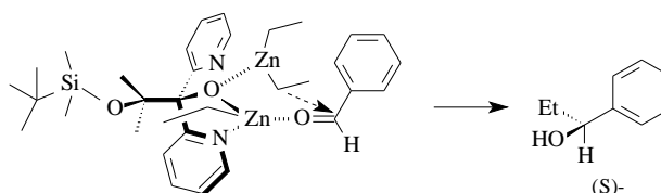
Scheme 10. The mechanism of benzaldehyde alkylation into the (S)-alcohol by Et 2 Zn.
