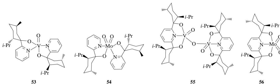
Figure 10. Multidentate catalysts for regioselective epoxidation.
