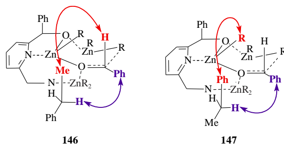
Scheme 12. Pyridine ring chelation and re -face attack of benzaldehyde by EtZn.
