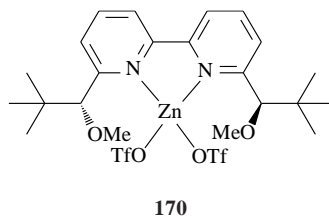
Figure 38. Chiral Zn-bipyridinyl complex.
