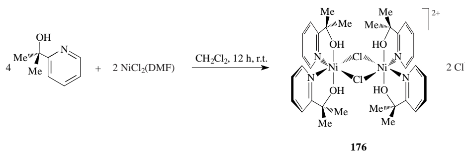
Scheme 24. Synthesis of complex 176 .
