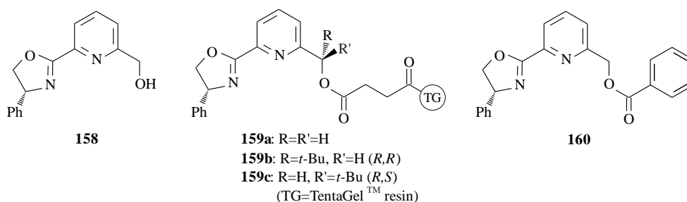
Figure 34. Unsupported and polymer-supported chiral pyridinooxazoline ligands.
