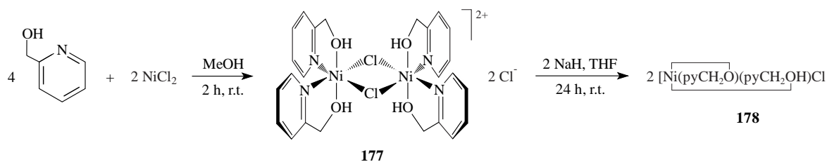
Scheme 25. Synthesis of complexes 177 and 178 .
