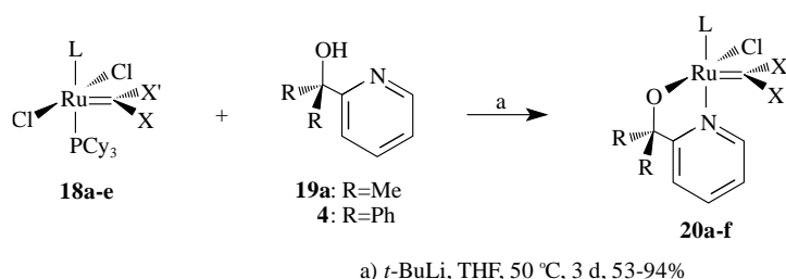
Scheme 3. Synthesis of pyridinyl alcoholato ligands from Gr1 and Gr2 ruthenium carbenes.
