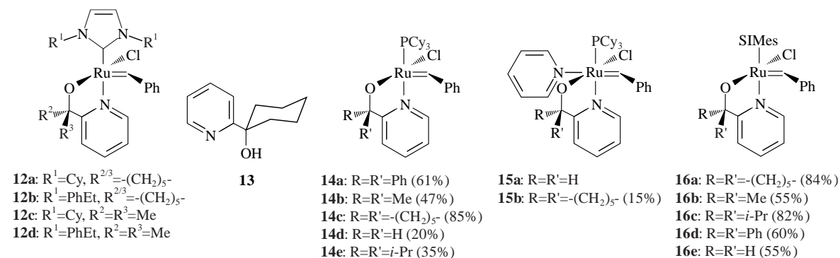
Figure 4. Pyridinyl alcoholato ruthenium carbene complexes.
