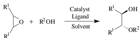
Scheme 16. A generalised ring-opening reaction of meso -epoxides by alcohols.
