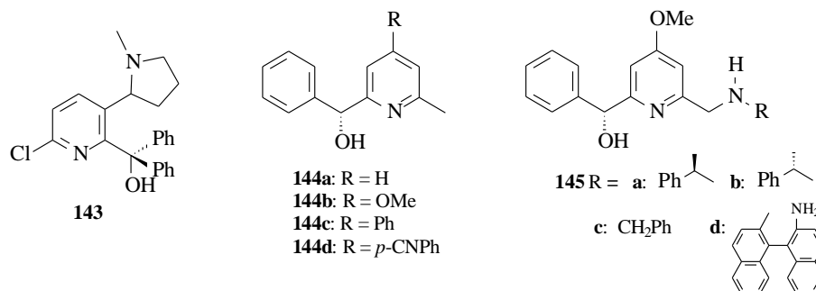
Figure 29. Pyridinyl alcohol compounds substituted on the pyridinyl group.
