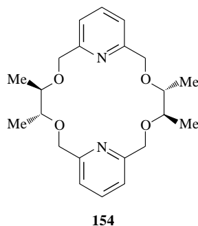
Figure 32. Pyridino-crown-ether synthesized from 2,6-pyridine dimethanol.
