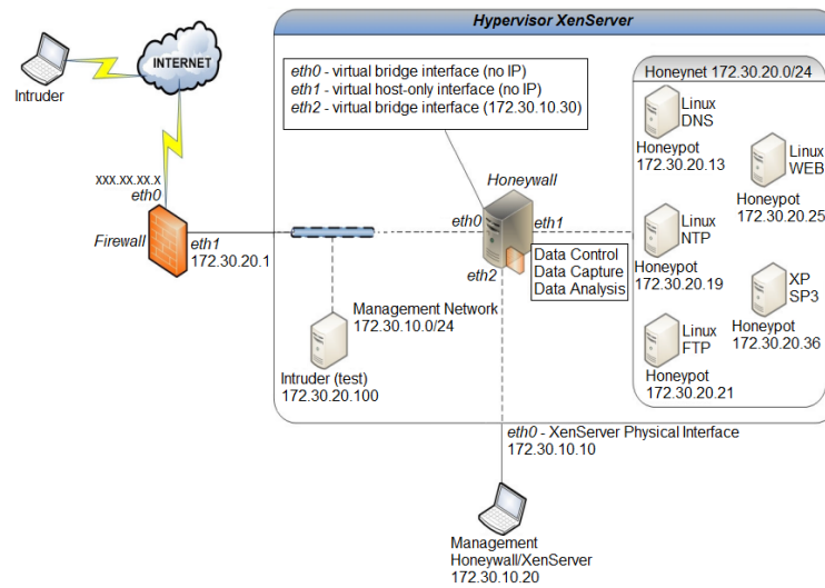
Figure 3. Honeynet architecture. [67].
