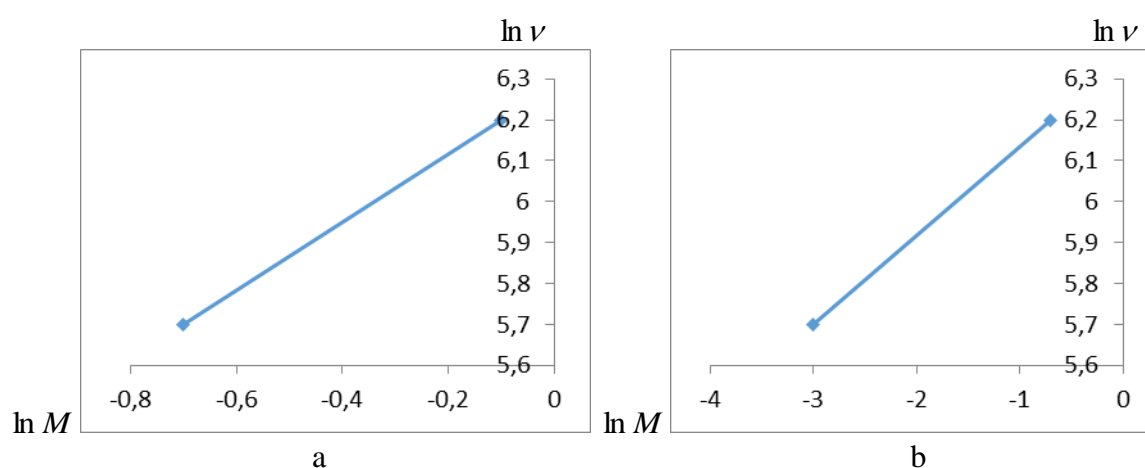
Fig. 3. Correlation between \nu and M at the temperatures of test (a) – 20, (b) – 120°C
