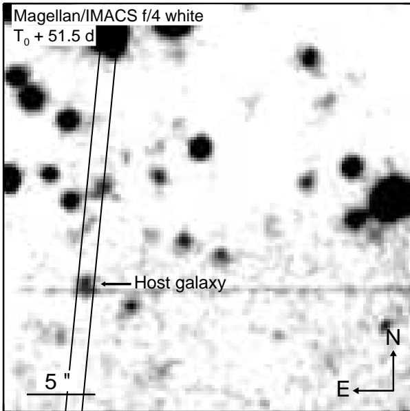
Fig. 1. Field of GRB 140506A ( 30'' \times 30'' ). The position of the host galaxy is marked. The slit of the late-time spectrum was inclined by -5^\circ 5' East of North. The image has been smoothed with a Gaussian kernel to increase the visibility of the host galaxy.
