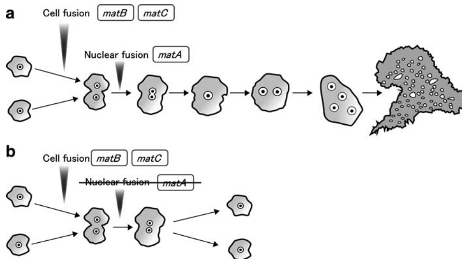
Fig. 2 Genetic control of zygote formation in the mating of Physarum polycephalum . a matA - , matB - , and matC - -heteroallelic cross. b matA -homoallelic cross. Zygote formation is under the control of three loci: matA , matB , and matC , with at least 16, 15, and 3 alleles, respectively. In the matB - or matC - -homoallelic cross, the two amoebal cells cannot fuse. The matA locus controls nuclear fusion in the fused cell of the matB - and matC - -heteroallelic cross.
