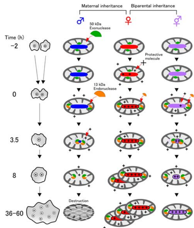
Fig. 9 A model for the molecular mechanism of mitochondrial inheritance in P. polycephalum . A 50-kDa exonuclease exists in the mitochondria of myxamoebal cells prior to mating. There is a complicated hierarchy in the multiallelic matA locus, but we think the paternal and maternal cells (indicated as ♂ and ♀, respectively) are just determined during cell–cell recognition. After recognizing the amoebal cell of another matA allele, the maternal cell begins to express (or activates) protective enzymes against endonuclease activity (protective molecules are indicated by plus). Shortly after cell fusion, the 13-kDa endonuclease is expressed in the zygote and is imported into each mitochondrion. The unprotected circular mtDNA of lower matA origin is cleaved by this endonuclease, and the 50-kDa exonuclease complex then digests it completely. Because the maternal mtDNA is protected against nuclease, it survives. This concerted digestion of mtDNA by these two nuclease activities leads to the uniparental inheritance of mtDNA. The delayed expression of endonuclease or the accelerated protection of some mtDNA molecules of lower matA origin in the zygote would result in the biparental inheritance of mtDNA (indicated as ♀ and ♂)
