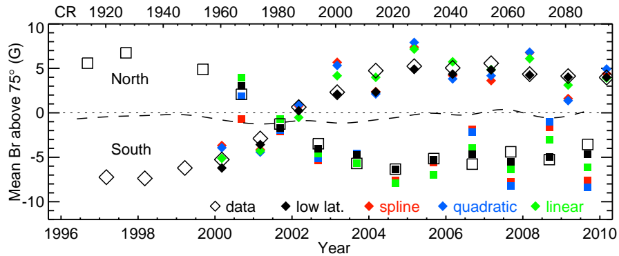
Figure 3. Comparison of four extrapolation methods for estimating the polar field strength of the next year: average from low-latitudes, cubic spline, quadratic and linear. Open squares (diamonds) indicate smoothed and averaged polar field flux density above 75° latitude in the north (south) during September (March). Each extrapolated point is based only on the data points before it. The low-latitude data are the average of the flux-density between 62° and 75° multiplied by 1.1, from the previous year. The dashed curve shows the average field strength difference between two poles after smoothing and averaging, which represents the residue imbalanced flux from polar field after the correction.
