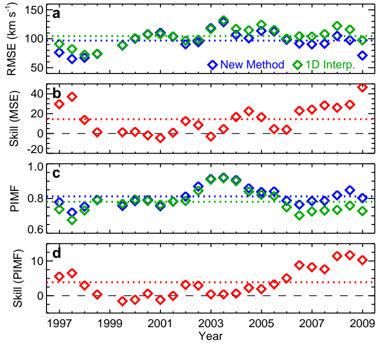
Figure 4. Statistical metrics for WSA solar wind speed and IMF polarity prediction compared with OMNI data. Results from synoptic maps with new polar field correction scheme are compared with those that use one-dimension interpolation. Each point represents a one-year window and the points are sampled every half a year. The overall average is shown as a horizontal dotted line. (a) Root mean square error (RMSE) from the new method (blue) and 1D interpolation method (green). (b) Skill score of mean square error (MSE) of the new method using the 1D method as reference. (c) Success rate of IMF polarity prediction (PIMF) from the new method (blue) and 1D interpolation method (green). (d) Skill score of the new method using the 1D method as reference.
