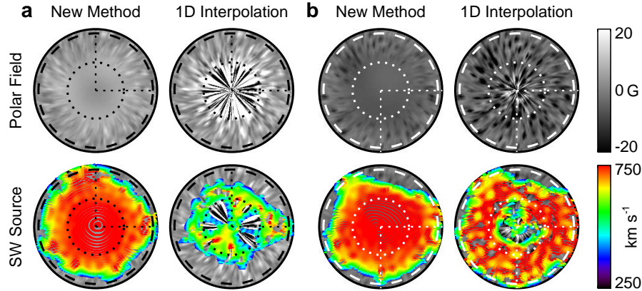
Figure 5. Comparison of derived open field line foot-points as the source location for high-latitude fast solar wind during solar minimum (CR1920), computed with new polar field correction and with 1D spatial interpolation method. (a) shows the North pole view. (b) show the South pole. In each panel, the top row shows the magnetic data after correction. The bottom shows the wind source overlotted on synoptic map, with colors indicating corresponding solar wind speed.
