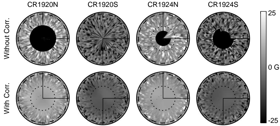
Figure 1. MDI synoptic maps of the radial field strength above 60° stereoscopically viewed from the poles: CR1920 (March 1997) and CR1924 (July 1997). In this projection, colatitude ( \theta ) increases with the distance ( R ) from the pole at the center of the circle as R \propto \tan \theta/2 , approximately linearly in this plot. Black indicates missing data. The top row shows the original data. The bottom row shows the field after interpolation. The small dotted circles indicate 75° latitude, the larger is at 62°. Horizontal solid lines show 0° Carrington longitude, vertical 90°.
