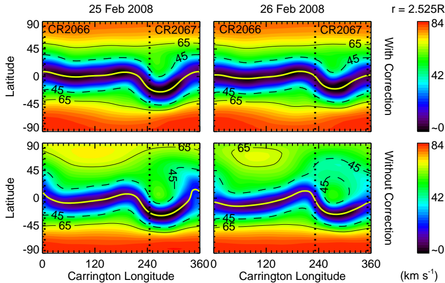
Figure 6. Solar wind speed distribution at the height of 2.525 R_{\odot} on 25 and 26 February, 2008, derived from a daily MHD simulation with MDI daily-updated synoptic maps as input. The top row is computed using maps with new interpolation. Maps used for the bottom row are not corrected. The Carrington longitude of the central meridian passage (CMP) for these two days are 305^{\circ} for and 292^{\circ} respectively. The leading edge of the map is 60^{\circ} east to the CMP and data within a 120^{\circ} longitudinal window centered at CMP (between the two dotted lines) is updated daily with new observations. In the speed contours, lines are drawn for values of 45 and 65 to highlight the high speed regions. Due to a few “bad pixels” in the north pole region of the updated data, great changes of the solar wind speed distribution are seen over one day. In addition, the typical high speed solar wind during solar minimum is missing from the North pole.
