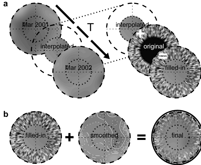
Figure 2. Illustration of the new polar field correction scheme. The circular plates are stereoscopic views of the South poles above 62° latitude. Smaller dotted circles indicate 75°. Black indicates missing data. Panel (a) shows the step of estimating the poorly measured pole-most pixels at a certain instant between March 2001 and March 2002 above 75°. The temporally interpolated values are used to replace the pole-most pixels in observation. Panel (b) shows the process of smoothly merging the filled-in data back to the map. The observed field with gap filled is smoothed and merged back to reduce the noise level in a standard way.
