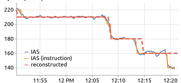
Figure 1: Trajectory of an aircraft landing at Zürich airport (SWR563 on November 28th, 2019), with the corresponding navigational points, altitude and speed settings; and the reconstructed trajectory in dashed lines.
