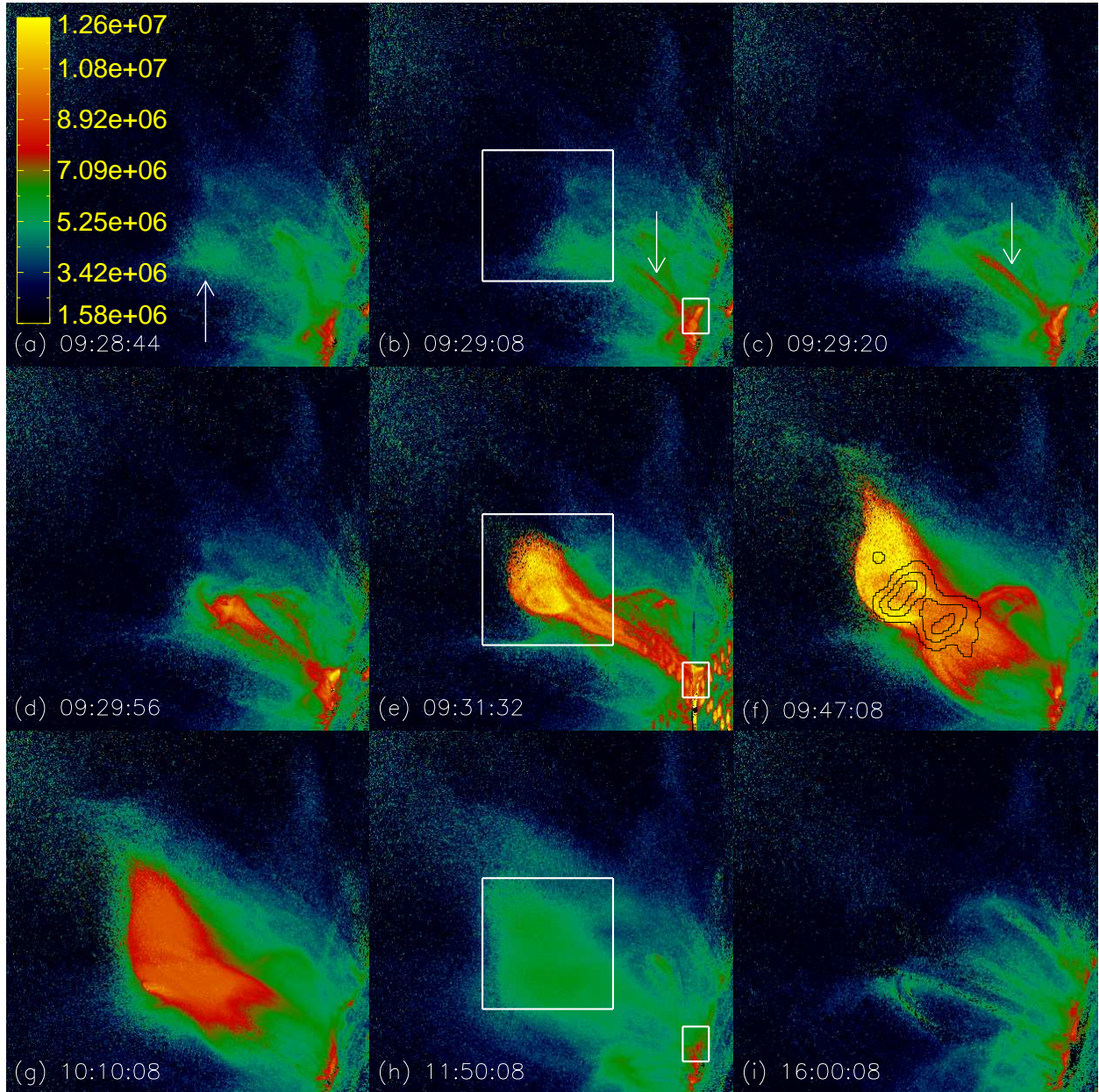
Fig. 2.— Temperature evolution process of the failed flux rope eruption. The FOV is the same as in Figure 1. (Animations of the full evolution of the temperature maps and a color version of this figure are available in the online journal.)
