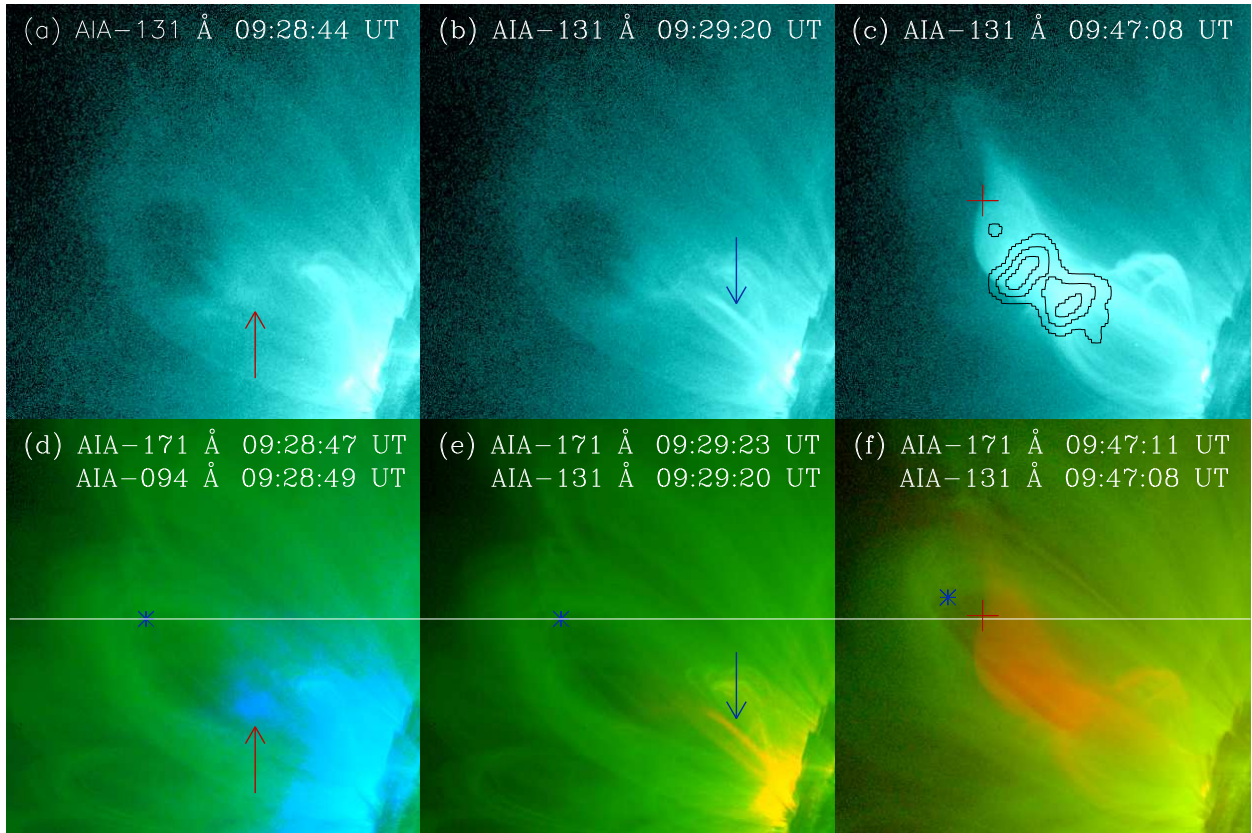
Fig. 1.— The failed flux rope eruption on 2013 January 5. The FOV is taken to be [-1140, -890] and [320, 570] arcsec for the horizontal and vertical axis, respectively. (Animations of the eruption process with full AIA cadence and a color version of this figure are available in the online journal)
