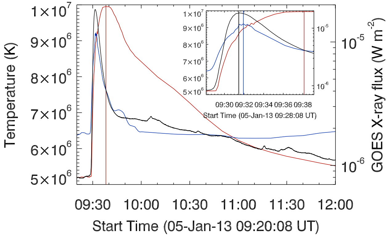
Fig. 3.— The temperature-time profiles of the high-lying flux rope (red) and the low-lying flare loops (blue), along with the profile of GOES soft X-ray 1-8 Å flux (black). (A color version of this figure is available in the online journal.)
