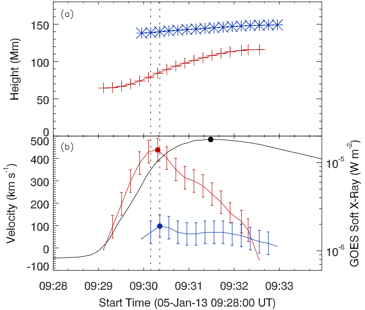
Fig. 4.— (a) The height-time profiles of the flux rope (red) and the loop arcade (blue). (b) The velocity-time profiles of the flux rope (red) and the loop arcade (blue), along with the profile of GOES soft X-ray 1-8 Å flux. (A color version of this figure is available in the online journal.)
