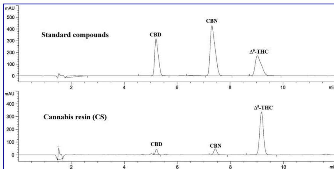
FIG. 2. HPLC chromatograms of the standard mixture of CBD, CBN, and \Delta^9 -THC (100 \mu\text{g/mL} ) and CS (200 \mu\text{g/mL} ). CBN, cannabinol; CS, cannabis resin; HPLC, high-performance chromatography.
