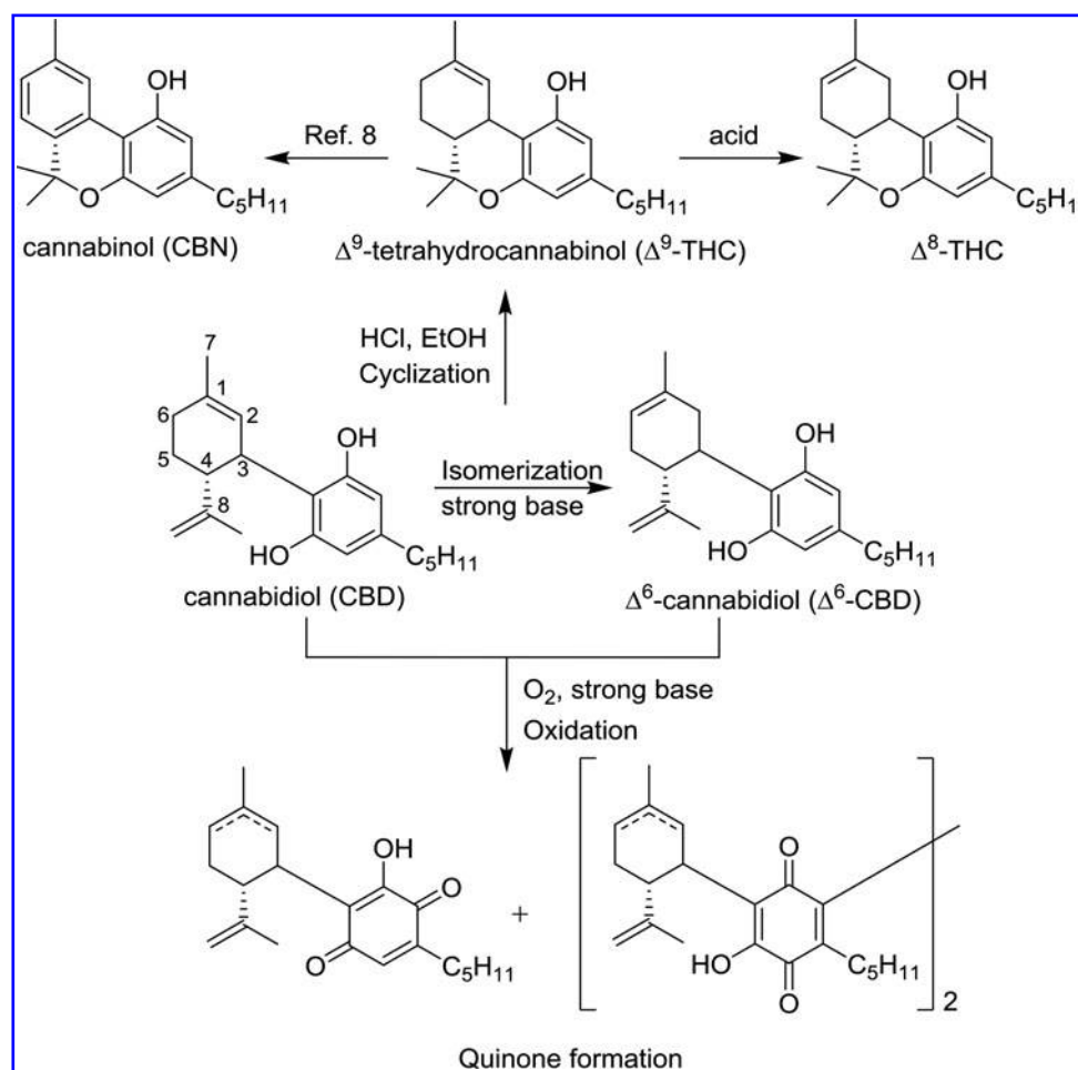
SCHEME 1. Chemical reactions of \Delta^9 -THC and CBD under acidic and basic conditions.
