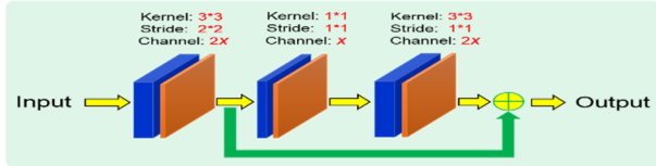
Figure 2: Demonstration of our residual block containing three convolution layers. This residual block is the basic unit of our HOREsNet network and is denoted as a green block in Fig. 3.
