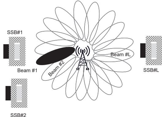
Fig. 1. Omnidirectional beam sweeping adopted for initial access in 5G NR, where each beam transmits the same SSB and up to L = 64 beams are supported in the FR2 band to cover the 360^\circ angular space [15].
