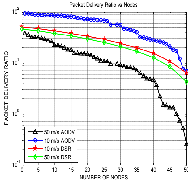
Fig.1 Packet delivery ratio vs. no. of nodes for speed 10m/s and 50m/sec
