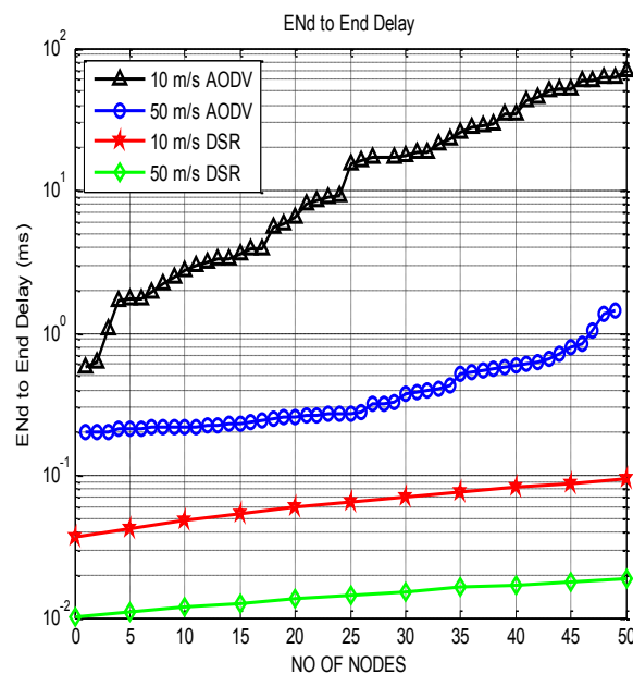
Fig. 4 End to end delay vs. no. of nodes for speed 10m/s to 50m/sec
