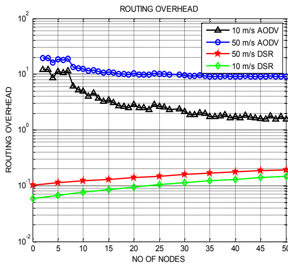
Fig.5 routing overhead vs. no. of nodes for Speed 10m/sec and50m/s.
