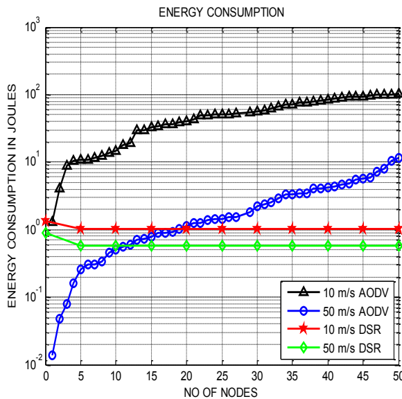
Fig.6 Energy consumption vs. no. of nodes for speed 10m/sec and 50m/s
