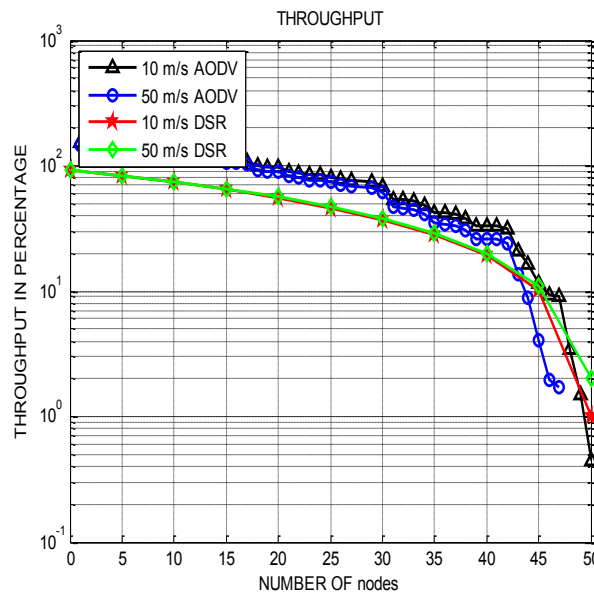
Fig.3 Throughput vs. no. of nodes for speed 10m/s and 50m/sec
