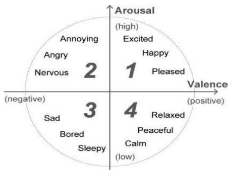
Figure 5. Sentiment Classification
