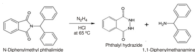
Scheme-II: Synthesis of 1,1-diphenylmethanamine
