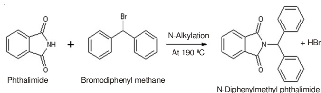
Scheme-I: Synthesis of N-diphenylmethyl phthalimide
