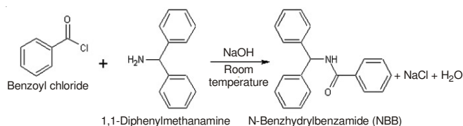
Scheme-III: Synthesis of N-benzhydrylbenzamide
