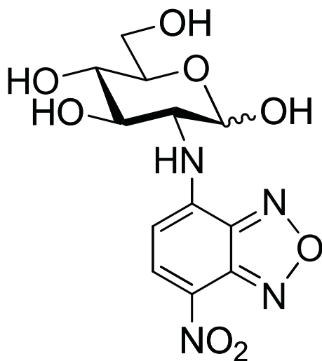
Fig. 1. 2-[N-(7-nitrobenz-2-oxa-1,3-diazol-4-yl)amino]-2-deoxy-D-glucopyranose (2-NBDG).
