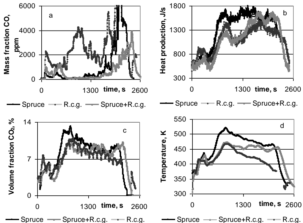
Figure 2: Time-dependent variations of (a) volatiles (CO) formation, (b) rate of heat energy production, (c) main product (CO 2 ) formation and (d) product temperature at the thermo-chemical conversion of densified biomass under stoichiometric combustion conditions ( \alpha \approx 1 ) downstream the combustor.
