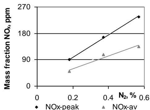
Figure 3: Correlation between the NO_x emissions and the nitrogen content in biomass samples.
