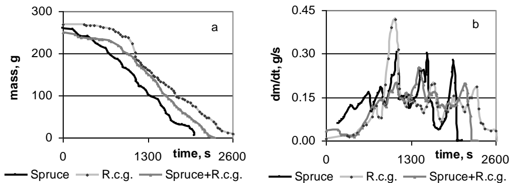
Figure 1: Time dependent variations of the mass loss (a) and mass loss rates (b) for different types of densified biofuels at the primary air supply rate 0.6 g/s.
