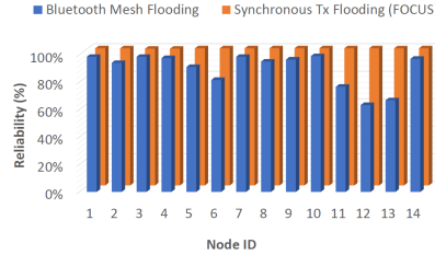
Figure 2. Synchronous flooding vs. Bluetooth Mesh
