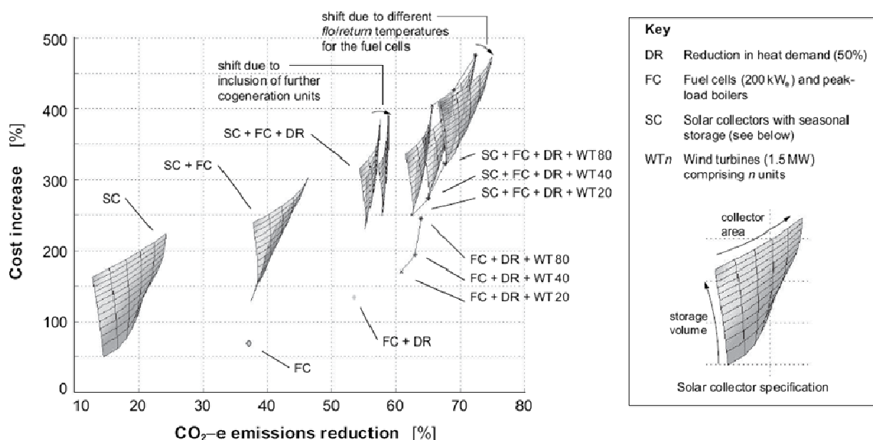
Figure 2.3 Feasibility analysis for 200 kW neighborhood fuel cells operating in a range of configurations and control settings.
