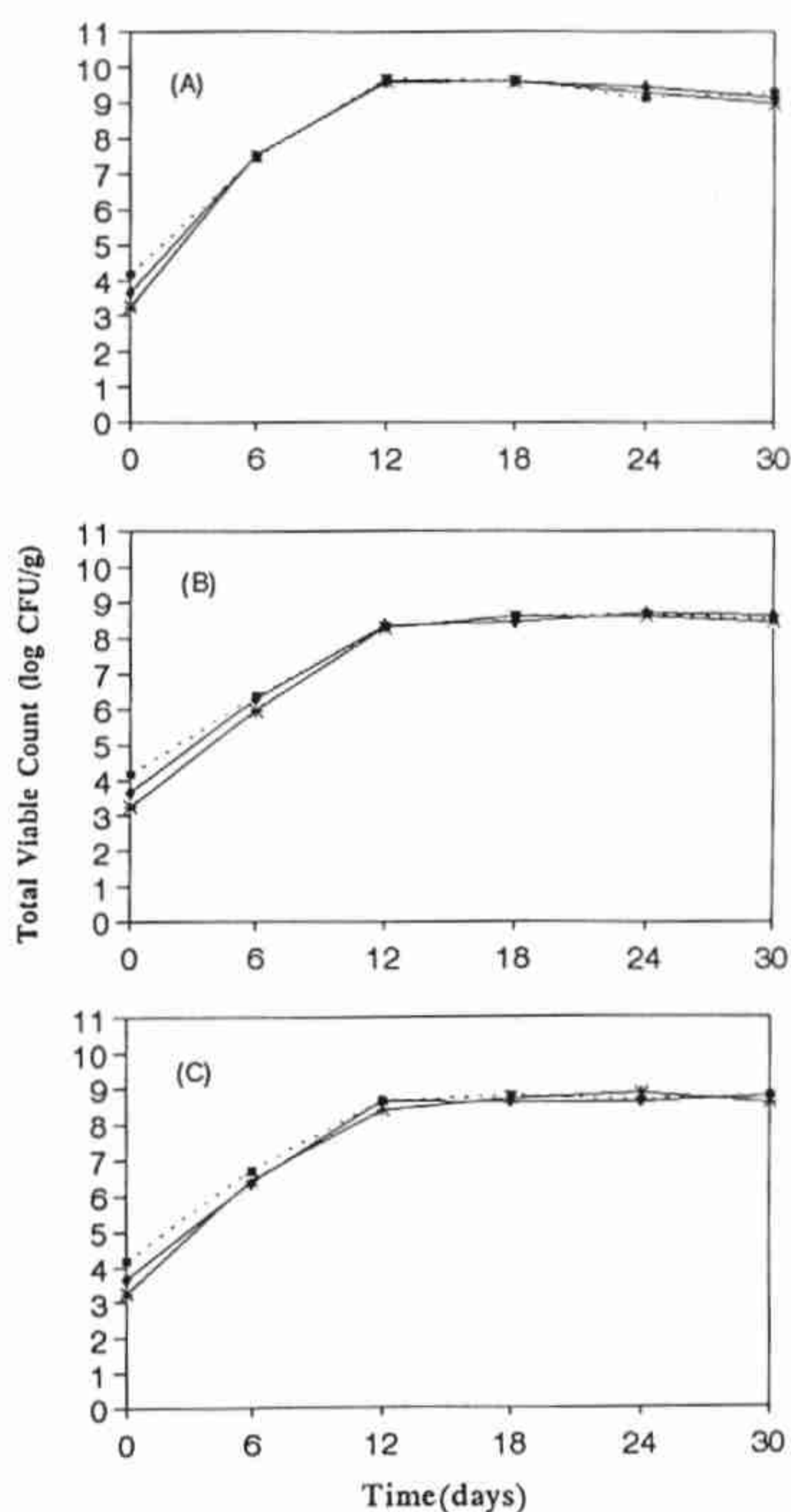
Figure 4. Effect of nisin concentration and packaging atmosphere on the growth of total aerobic counts when stored in air (A), 100% CO 2 (B), and 80% CO 2 + 20% air (C). Nisin concentration: 0 IU/ml (-■-), 10^4 IU/ml (◆), and 5 \times 10^4 IU/ml (≍) at 4°C.
