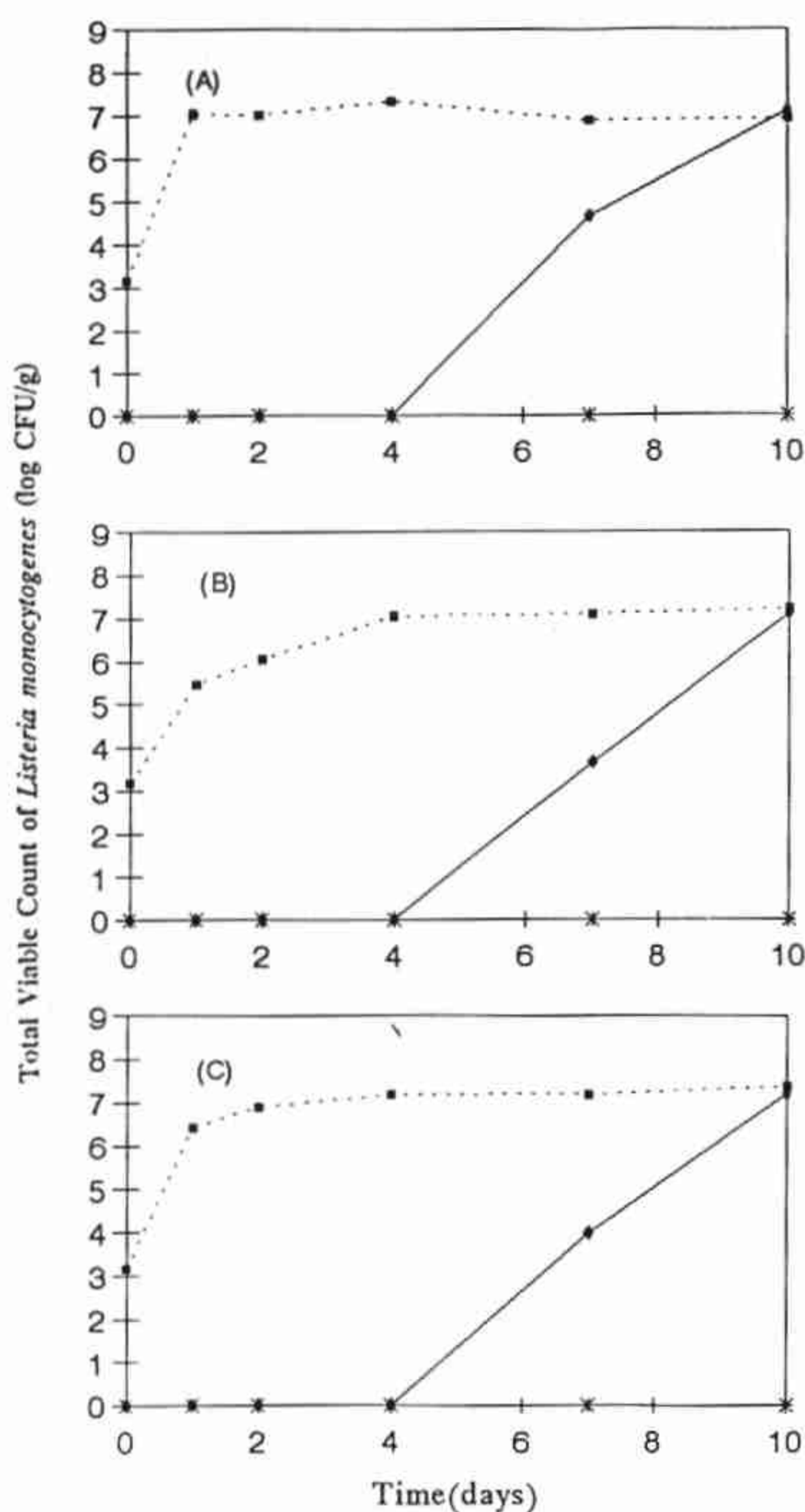
Figure 3. Effect of nisin and packaging atmosphere on the growth of L. monocytogenes when stored in air (A), 100% CO 2 (B), and 80% CO 2 + 20% air (C). Nisin concentration: 0 IU/ml (-■-), 10^4 IU/ml (◆), and 5 \times 10^4 IU/ml (≍) at 20°C.
