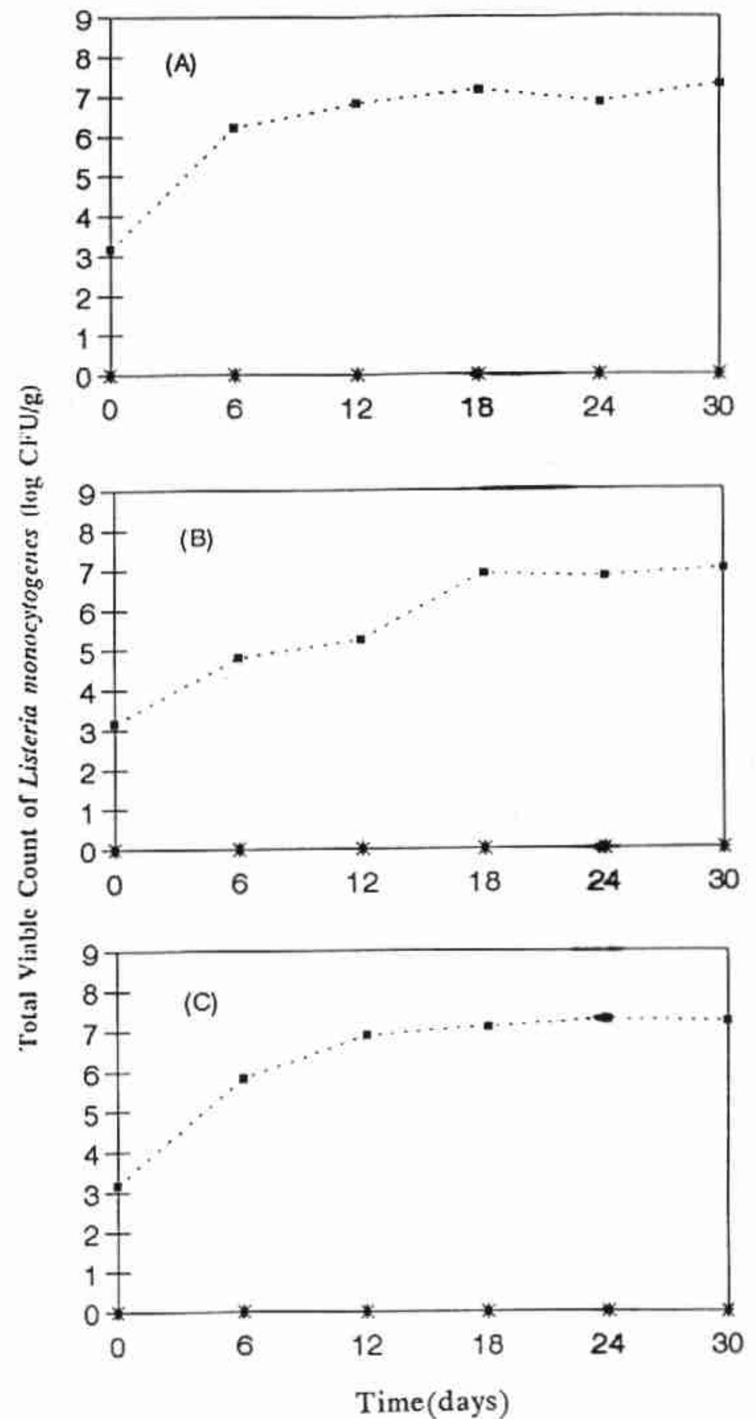
Figure 2. Effect of nisin and packaging atmosphere on the growth of L. monocytogenes when stored in air (A), 100% CO 2 (B), and 80% CO 2 +20% air (C). Nisin concentration: 0 IU/ml (■), 10 4 IU/ml (◆), and 5 × 10 4 IU/ml (✱) at 4 °C.
