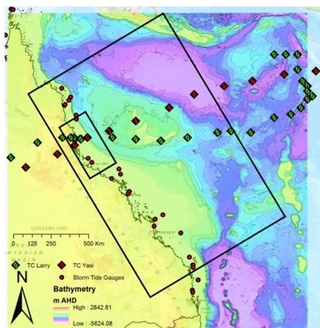
Figure 12: Regional modal extents of NQLDFM1 model with storm tide observation stations [5], 3DGBR bathymetry [10] and tracks of TC Larry and TC Yasi [1]
