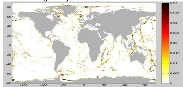
Figure 2 Distribution of barotropic energy dissipation through the generation of internal waves for one month, using the new parameterization (W/m2). As expected, the dissipation is concentrated around ocean ridges, continental shelves and island chains in deep water.
