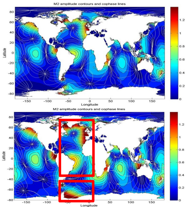
Figure 4: M2 Co-tidal chart for FES2012 benchmark in global tidal models (top) and GTSM (bottom) show a clear misrepresentation close to the ice-covered seas and an over prediction in the Atlantic ocean.
