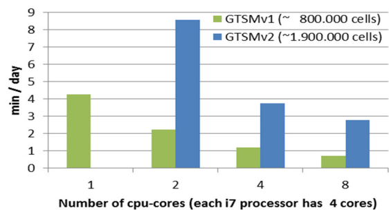
Figure 6: GTSMv2 and v1 computation times on a cluster; wall-clock in minutes per simulation day
