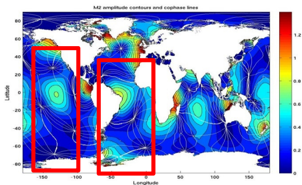
Figure 5: M2 Co-tidal chart for GTSM model including bathymetry below the permanent ice shelves shows clear improvements, especially for the Atlantic and Pacific Oceans due to improved bathymetries for the Weddell and Ross Seas, respectively.
