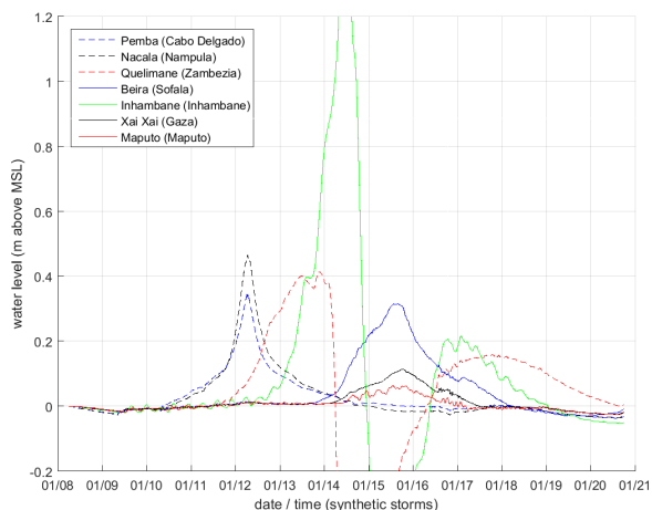
Figure 11: Time series of storm surge, for synthetic storm #366 in the stochastic experiment, at each of the seven coastal province capitals
