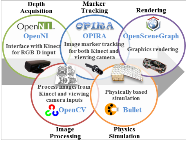
Figure 2: Primary components of our framework and the underlying software libraries.
