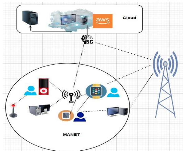
Figure 4: Cloud-MANET mobility model
