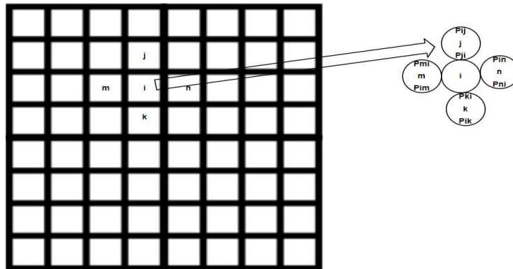
Figure 2: HMM model transition matrix representation
