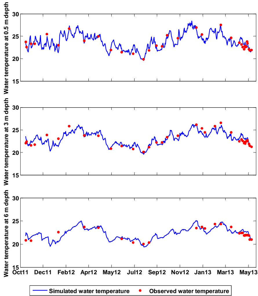
Figure 1 : Simulated (line) and observed (dots) water temperature in Lake Pampulha (point P1) at 0.5 m, 3.0 m and 6.0 m depth from October 18 th 2011 to June 04 th 2013.
