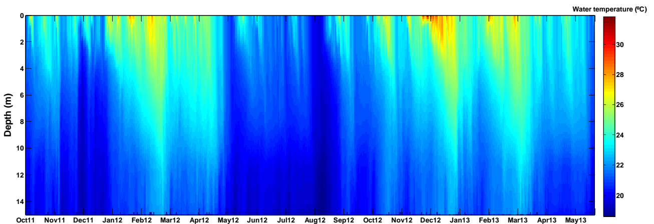
Figure 2 : Vertical variations of water temperature simulated by the GLM in Lake Pampulha (point P1) from October 18 th 2011 to June 04 th 2013.
