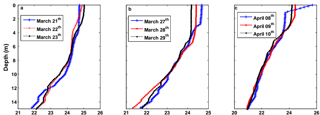
Figure 4: Vertical profiles of water temperature simulated by the lake model at Point P1. a – Rain event on March 22 th ; b – Rain event on March 27 th ; c – Rain event on April 08 th .
