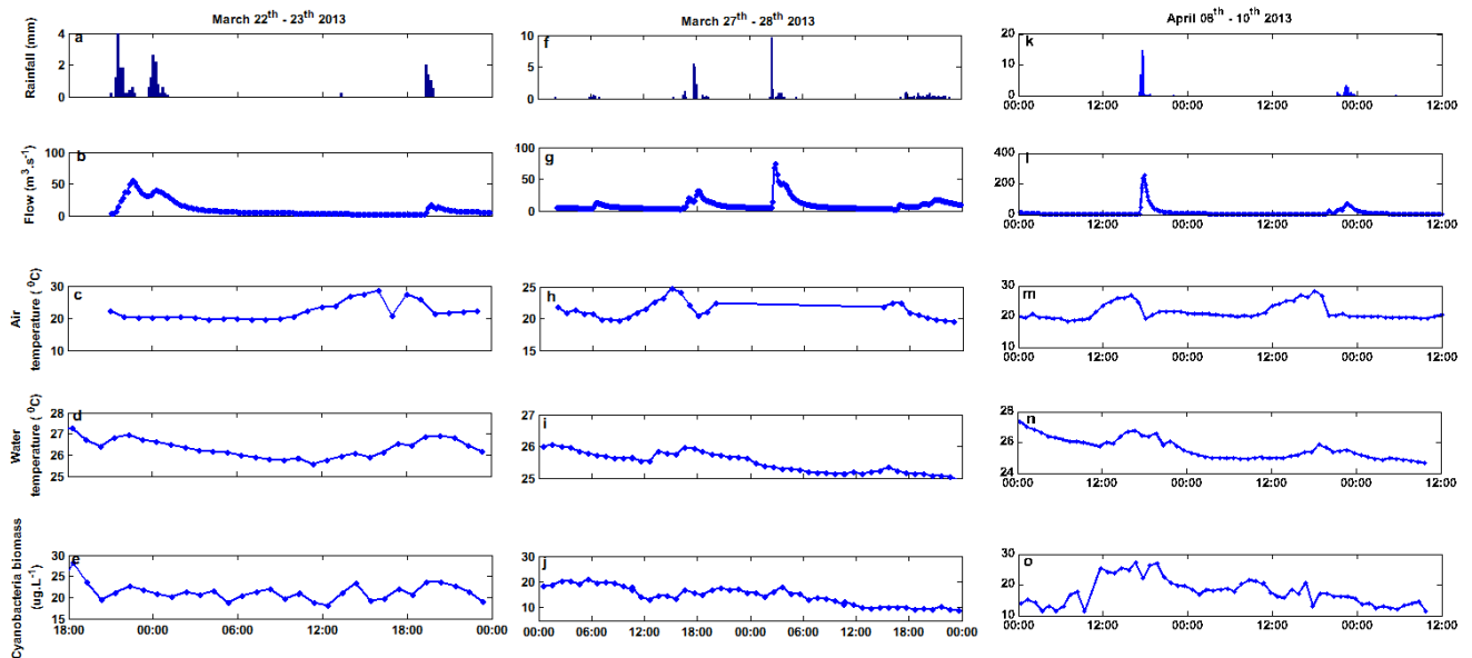
Figure 3: Stormwater runoff impacts on water temperature and cyanobacteria dynamics. a, f and k - Rainfall (mm); b, g and l – inflow into Lake Pampulha (m 3 .s -1 ); c, h and m – Air temperature (°C); d, i and n – water temperature from SMATCH buoy (°C); e, j and o – cyanobacteria biomass (µg chl-a. L -1 ).
