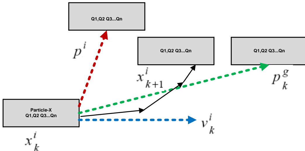
Figure 2 PSO mechanism over N-Queens problem
