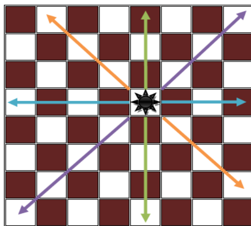
Fig 1 Queen Attacking Search Space
