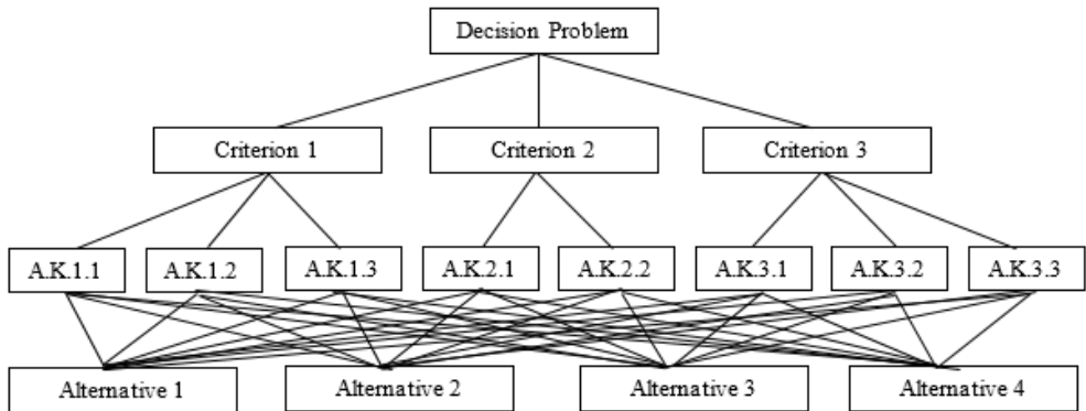
Figure 1: Hierarchical Structure of AHP
