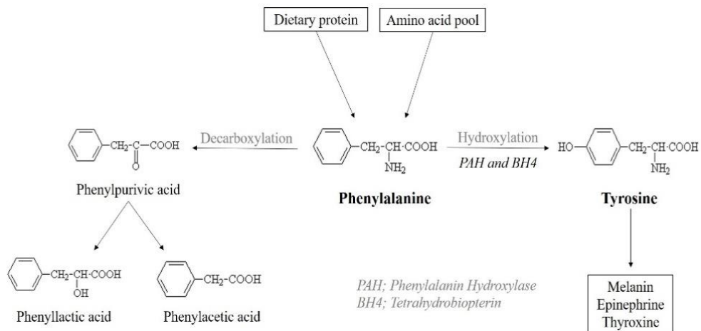
Figure 1. Metabolic pathways of phenylalanine
