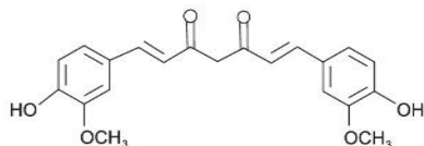
Figure 1: Chemical Structure of Curcumin
