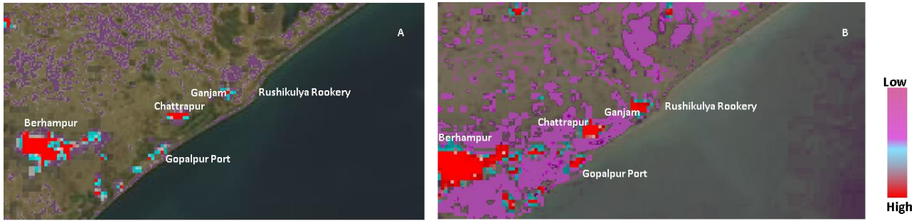
Fig 3 showing the illumination zones in rushikulya rookery during a) 2012 and b) 2016
