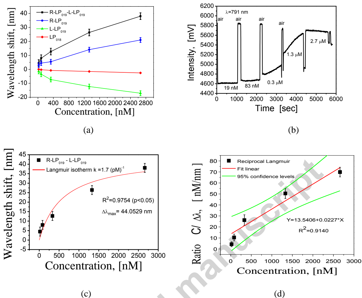
Figure 7. (a) Concentration dependence of the wavelength shift derived from the data shown in figure 6a; squares, wavelength differences between R-LP 019 and L-LP 019 resonance bands; circles, R-LP 019 band; triangles, L-LP 019 resonance band; and diamonds, LP 018 resonance band. (b) The change in transmission of the device measured at a wavelength of 791 nm on immersion into solutions of different SV concentration. (c) Langmuir isotherm fit of data from figure 7a and (d) linearization of Langmuir isotherm (Figure 7c) using Eq. 4. The error bars represent the standard deviation of 5 blank measurements and the green lines provide the confidence level (Belter et al., 2014; Lock and Wentzell, 2012).
