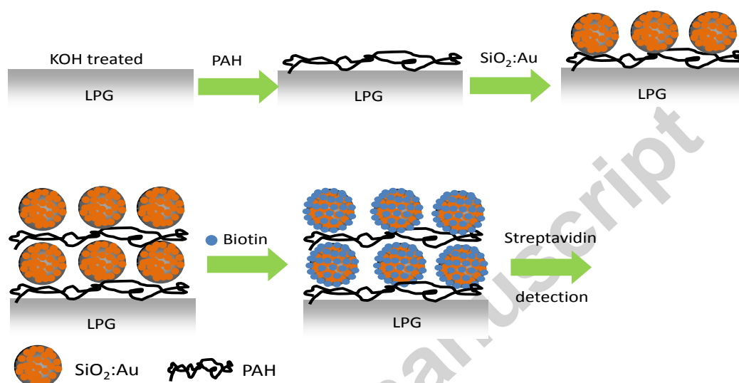
Figure 3. Schematic illustration of the layer-by-layer deposition of a (PAH/SiO_2: Au)_2 film onto an optical fibre LPG.
