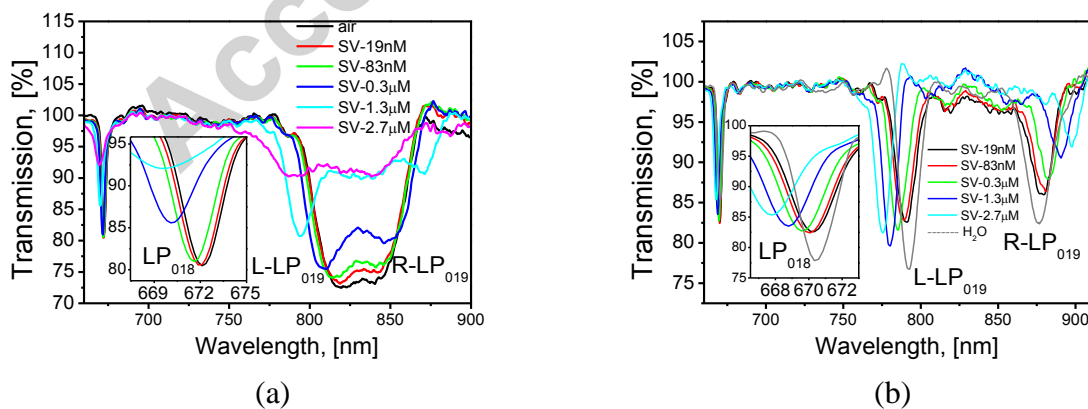
Figure 6. Transmission spectrum of the (\text{PAH}/\text{SiO}_2(300 \text{ nm}):\text{Au})_3 coated LPG modified on exposure to SV of different concentrations in: (a) air and (b) aqueous solution.
