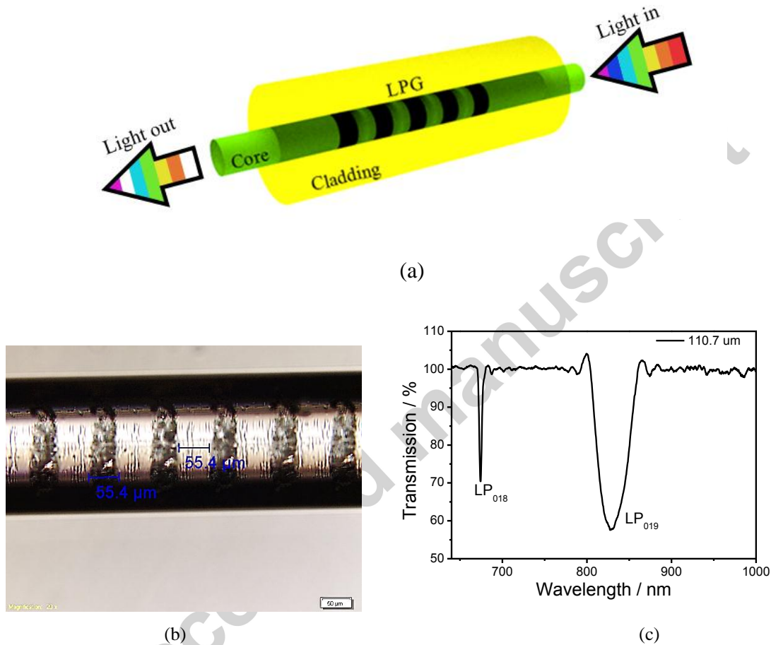
Figure 1: (a), schematic illustration of the LPG optical fibre; (b), optical image of the LPG written in the plastic jacket of the optical fibre; and (c), transmission spectrum (TS) of the LPG optical fibre operating at phase matching turning point (PMTTP) with the grating period of 110.7 \mu\text{m} measured in air.
