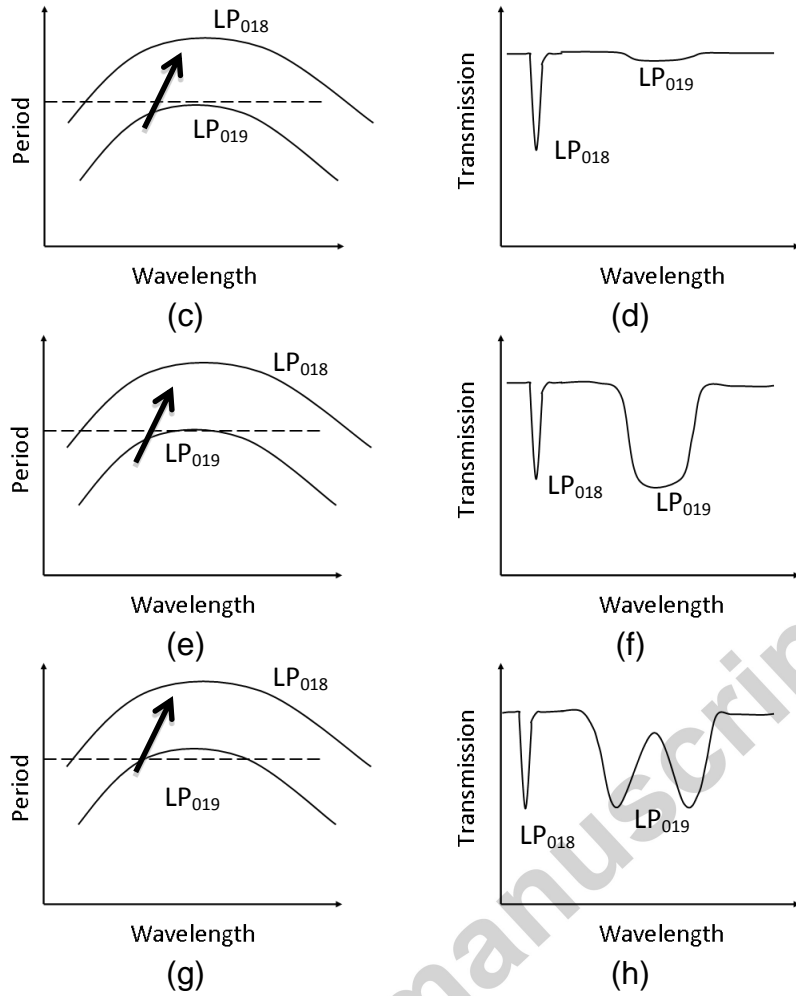
Figure 2. Illustration of the properties of an LPG near the PMTP; arrow shows direction of the shift of the phase matching curve at the increase of the effective refractive index of the cladding mode caused by increasing optical thickness.
