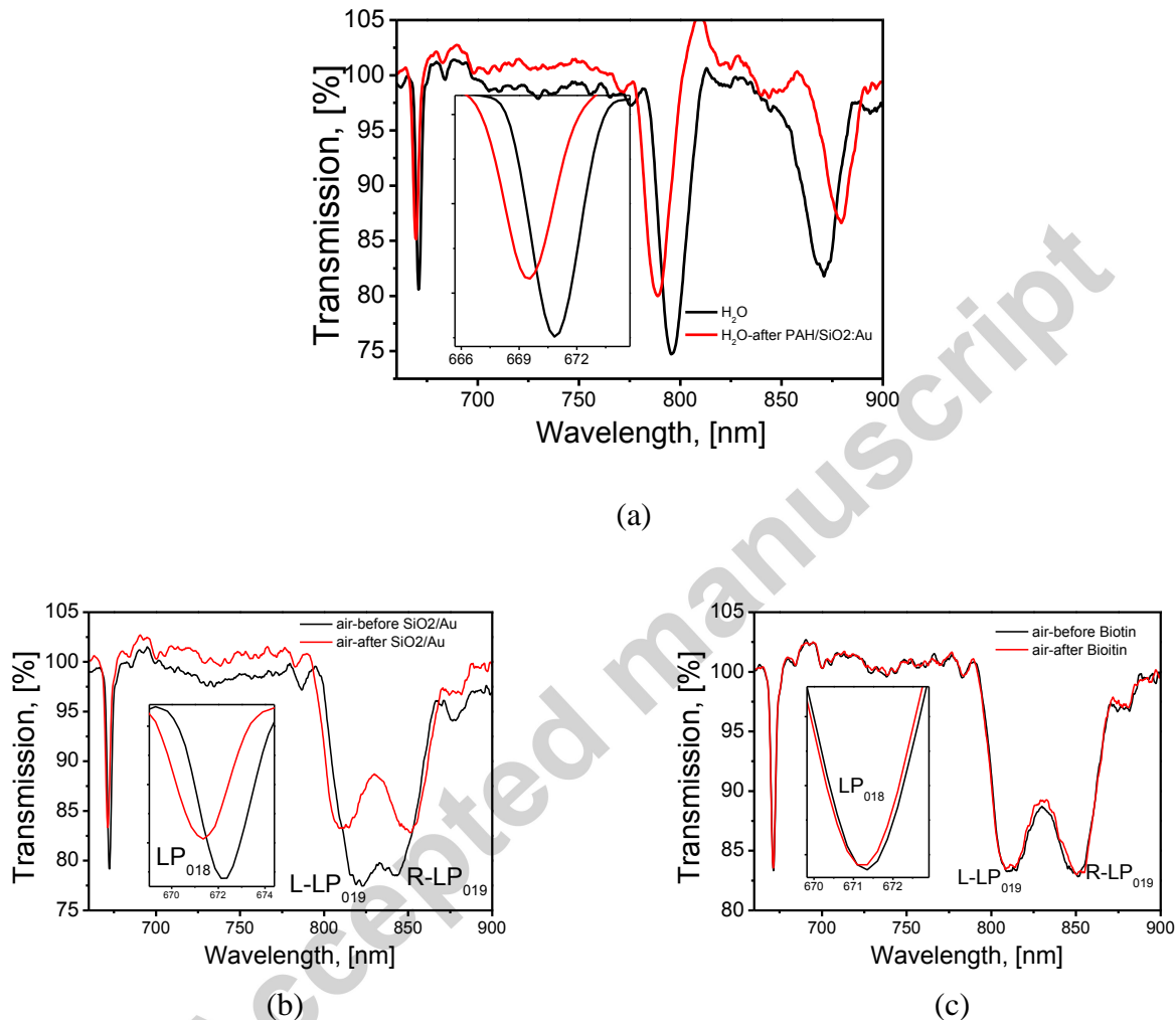
Figure 5. (a) The transmission spectrum of an LPG of period 110.7 \mu\text{m} , measured with the LPG in water and (b) in air: black line, before and red line, after (\text{PAH}/\text{SiO}_2(300 \text{ nm}):\text{Au})_3 film deposition; and (c) transmission spectrum of the LPG coated the (\text{PAH}/\text{SiO}_2(300 \text{ nm}):\text{Au})_3 film, measured with the LPG in air: black line before and red line, after biotin deposition.
