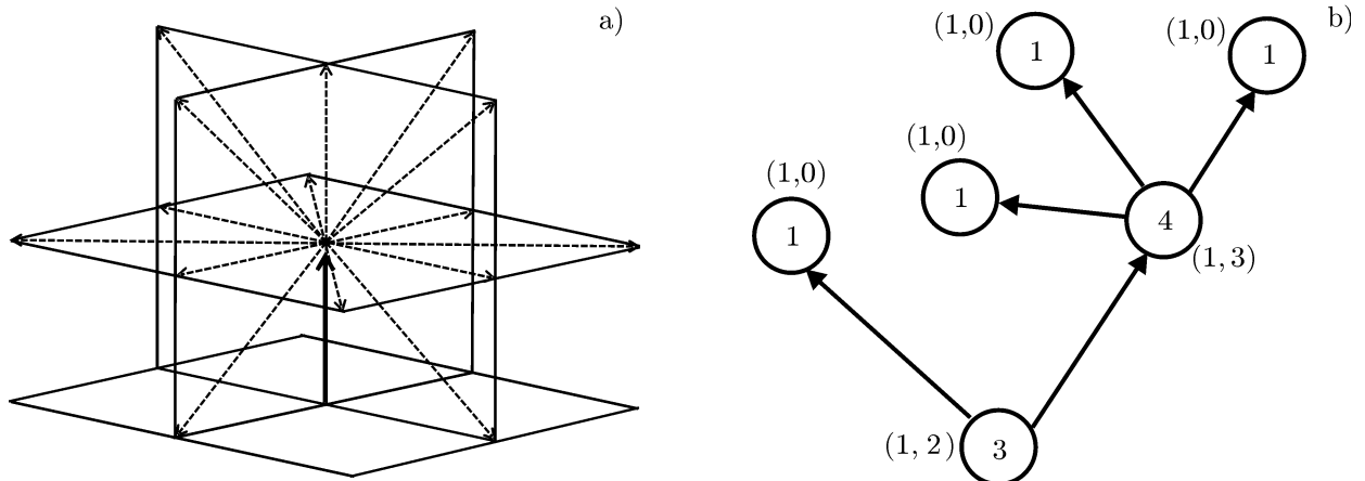
Fig. 1. Scheme of development of the discharge tree in three-dimensional space: (a) the possible directions of development from the active node; (b) the instantaneous state of the discharge graph. The circles correspond to the nodes of the conducting graph, and the inscribed numbers denote the node indices. The number of incoming and outgoing directed edges (arrows) for the given node is shown in the parentheses.
