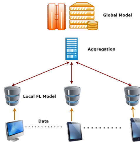
Figure. [5]: Fundamental FL Architecture
