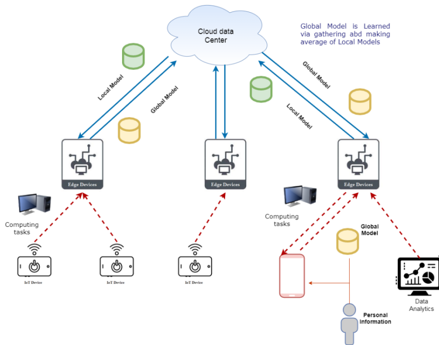
Figure [6]: Process of FL
