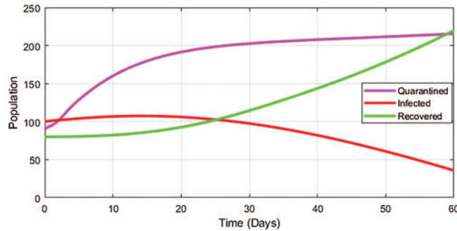
Figure 6: Dynamics of quarantined, infected and recovered individuals where recovered individuals are increased due to increase of quarantined individuals
