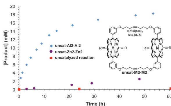
Fig. 2 Reaction profiles for the methanolysis of PNPDP carried out in the absence or presence of 3 mol% of unsat-Al2-Al2 or unsat-Zn2-Zn2 .
