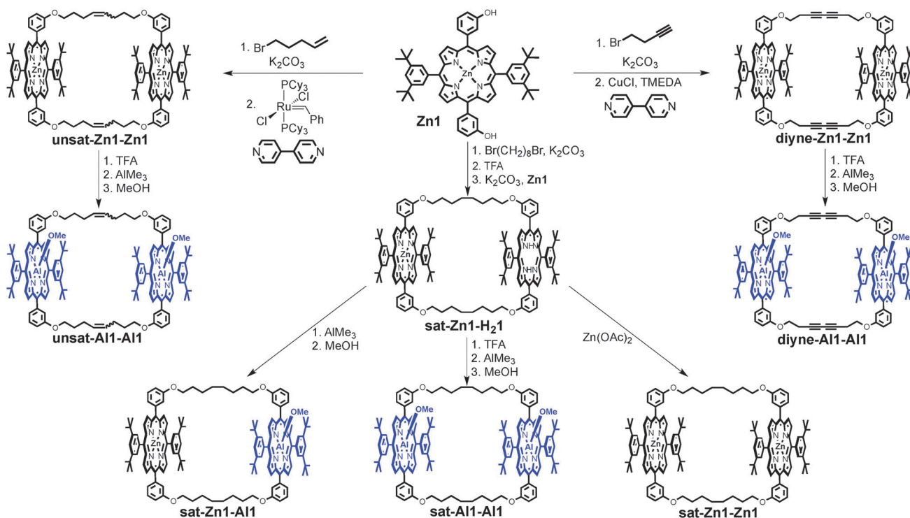
Scheme 1 Modular synthesis of catalytic porphyrin dimers starting from the same starting porphyrin monomer, Zn1 .
