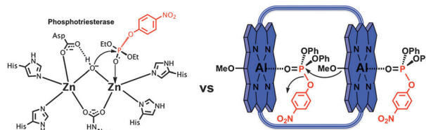
Fig. 1 Degradation of a phosphate triester in the active site of a phosphotriesterase enzyme 11 (left) and proposed catalytic methanolysis of a phosphate triester in an Al porphyrin dimer.
