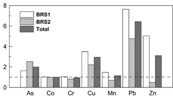
Fig. 4 Averaged enrichment factors for elemental soil data from the sample sets of BRS1, BRS2, and BRS1 and BRS2 together from Louisiana, USA
