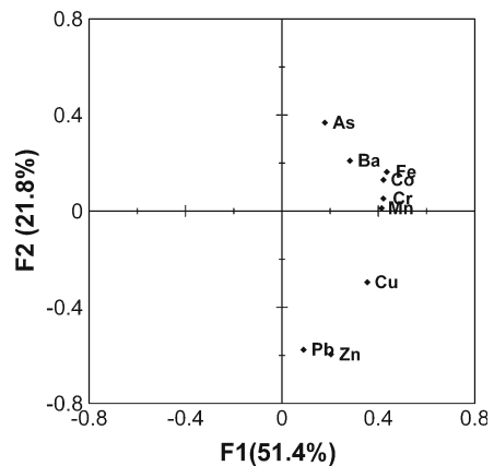
Fig. 3 Principal component analysis for all samples from sites BRS1 and BRS2 in Louisiana, USA
