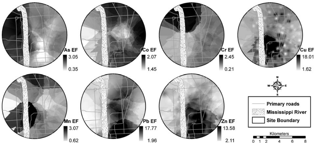
Fig. 5 Interpolated enrichment factor maps for selected elements at site BRS1 (Louisiana, USA) using ordinary kriging
