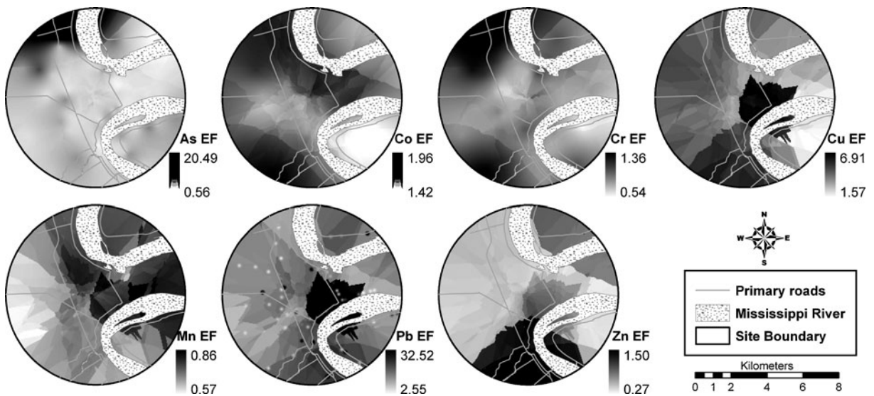
Fig. 6 Interpolated enrichment factor maps for selected elements at site BRS2 (Louisiana, USA) using ordinary kriging
