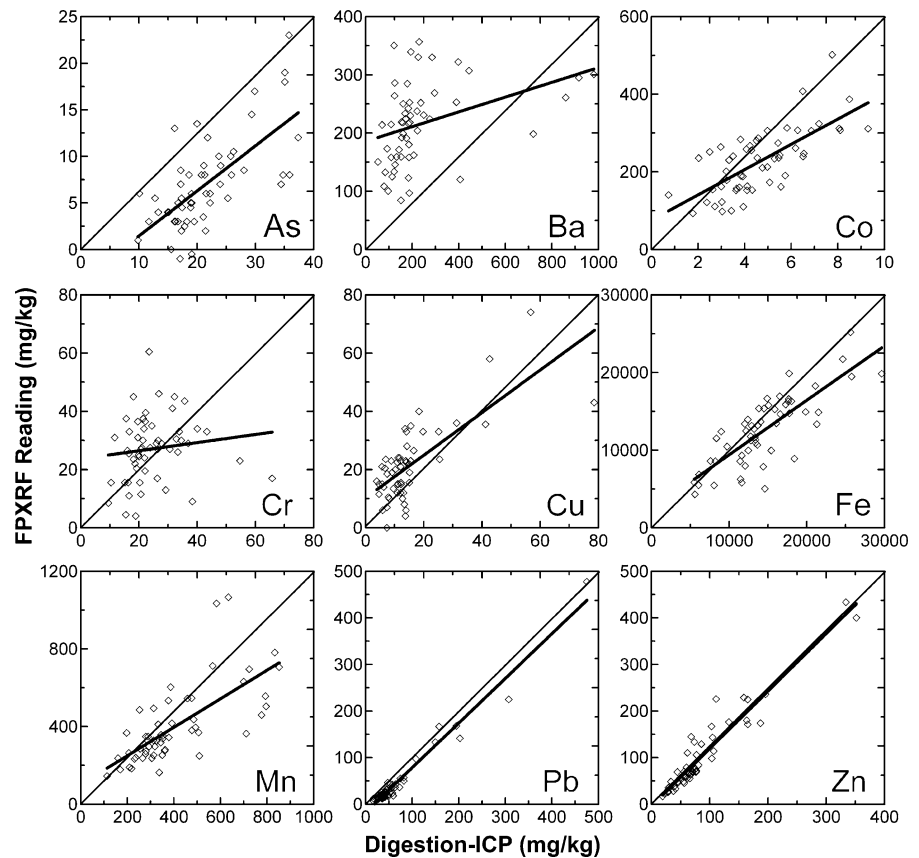
Fig. 2 Correlation between PXRF readings and aqua regia digestion–ICP results (with correction of field moisture contents) for the studied soil elements at two sites in Louisiana, USA
