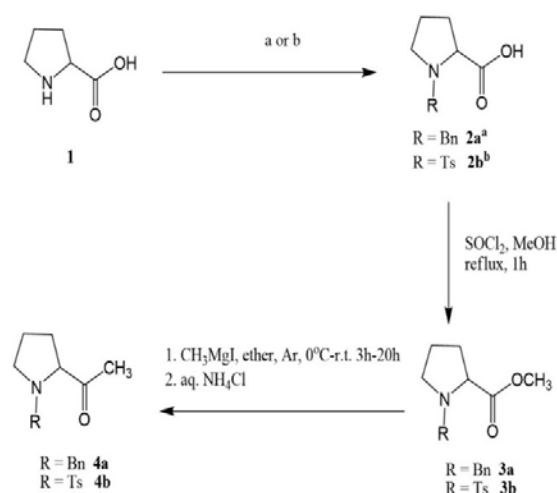
Scheme 1. Preparation of N -substituted-2-acetylpyrrolidine ( 4a-b ). DMF, N,N -dimethylformamide; a, 1. KOH, DMF, 0 °C, 10 min; 2. BnCl, r.t., 3 h; b, 1. 2M NaOH, 0 °C and 2. TsCl, 0 °C, 30 min, then 2M NaOH, room temperature, 24 h.
