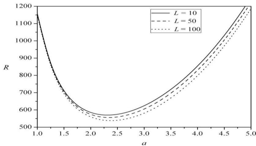
Fig. 3 Variation of thermal Rayleigh number R with a for different values of Roberts number L when C = 0.01 .
