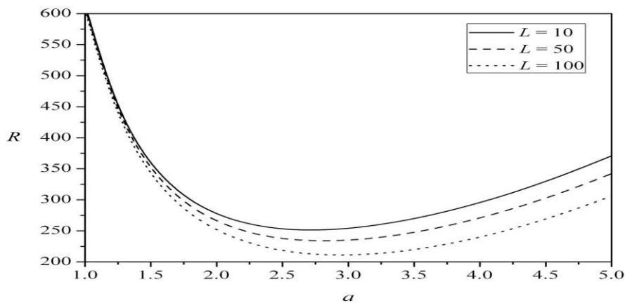
Fig. 4 Variation of thermal Rayleigh number R with a for different values of Roberts number L when C = 0.1 .
