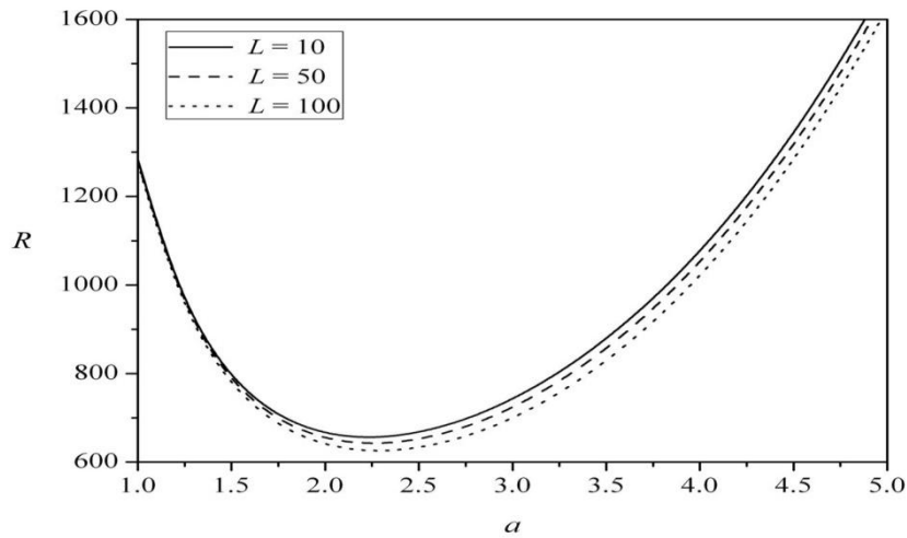
Fig. 2 Variation of thermal Rayleigh number R with a for different values of Roberts number L when C = 0 .
