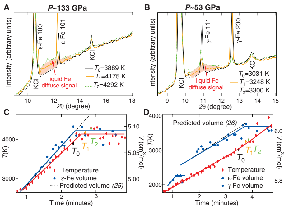
Fig. 1. XRD patterns as a function of temperature, pressure, and time. (A and B) XRD patterns of a ~3-µm-thick (~7-µm-thick) sample during a heating series at P \approx 133 GPa and 53 GPa, respectively, recorded at different temperatures. \gamma -Fe, \epsilon -Fe, and KCl pressure medium diffraction peaks are labeled. Liquid Fe is evidenced by a diffuse ring at 2\theta = 10^\circ to 13.5^\circ . (C and D) Pyrometry temperature, measured and predicted (25, 26). Fe volume as a function of time for the thin (C) and thick (D) samples. The laser’s power is linear with time. Data are in table S1.
