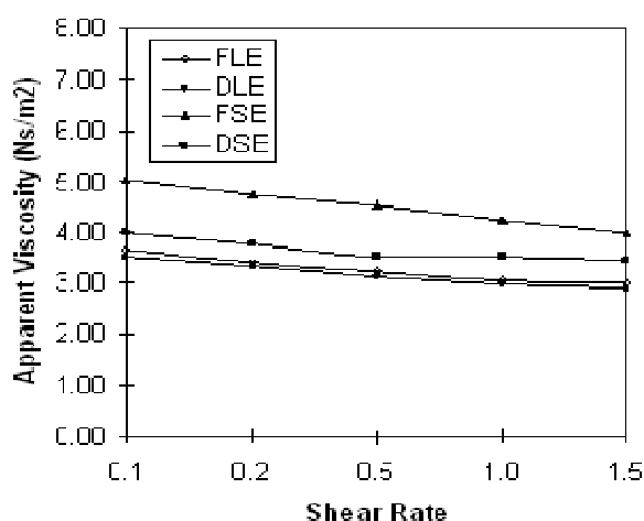
Figure 1. Apparent viscosity versus shear rate at 60°C.
