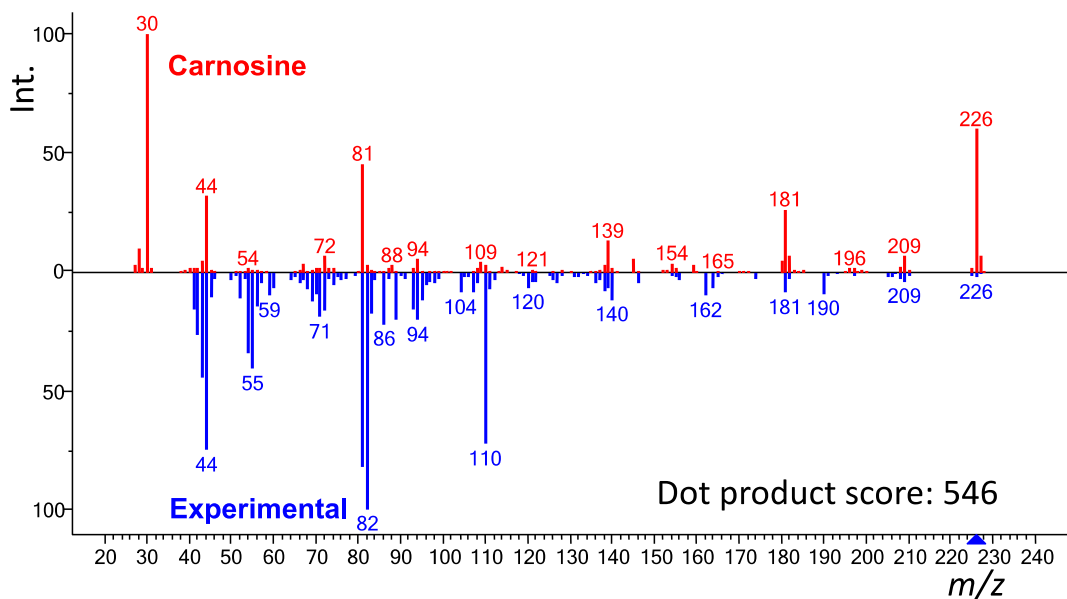
Figure 4-S5. Head-to-tail plot; Hybrid spectrum of carnosine against experimental spectrum from NIST17
