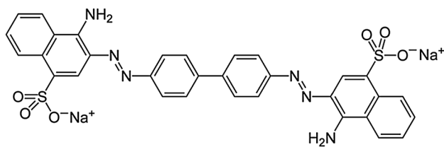
Fig. 1 Chemical structure of Congo red
