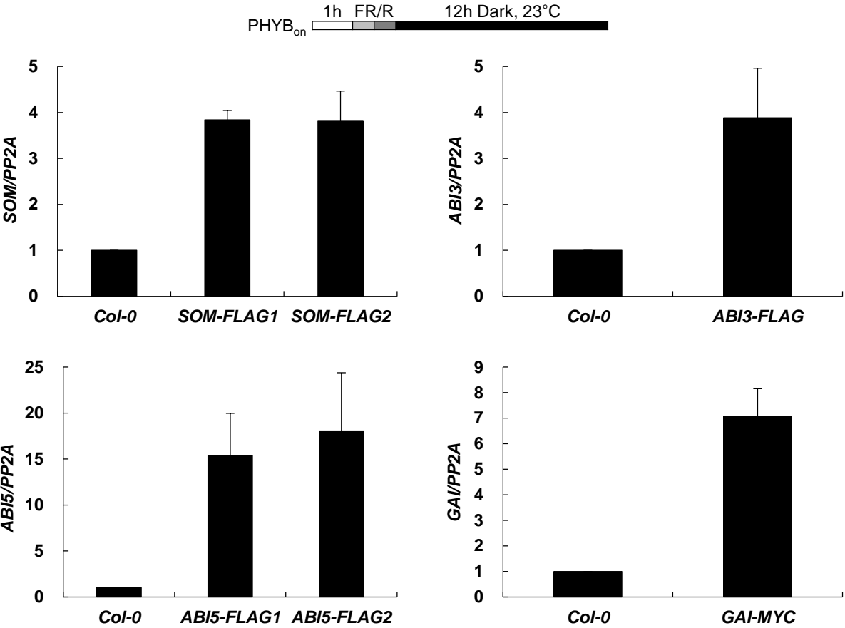
Supplemental Figure 1. mRNA expression levels of SOM , ABI3 , ABI5 , and GAI in corresponding overexpression lines. The top diagram indicates the light treatments and seed incubation condition. mRNA levels of each gene (endogenous + transgene) were normalized by mRNA level of PP2A and then by Col-0 expression levels. Error bars indicate the SD of three biological replicates (n = 3). SOM-FLAG1 , -FLAG2 , ABI3-FLAG , ABI5-FLAG1 , and -FLAG2 indicate 35S-driven FLAG-tagged overexpressing lines. GAI-MYC indicates a 35S-driven MYC-tagged GAI -overexpressing line.
