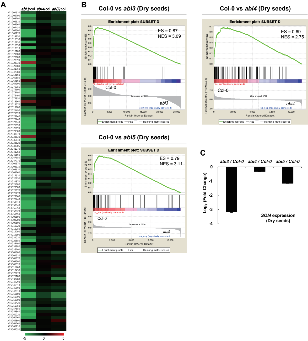
Supplemental Figure 6. Decreased expression of the subset D genes in the abi3 , abi4 , and abi5 mutant dry seeds. We analyzed microarray data reported previously (Nakashima et al. (2009) for abi3 ; Nakabayashi et al. (2005) for abi4 and abi5 ). (A) Heatmap analysis showing expression of the subset D genes in the abi3 , abi4 , and abi5 mutant seeds compared with Col-0 seeds. The color map index indicate fold changes ( \log_2 ). Abi3 data are average values of two biological replicates, while abi4 and abi5 data are values of one of two biological replicates. (B) GSEA indicating the repression of subset D genes in the abi3 abi4 , and abi5 mutant seeds (FDR < 0.001). ES: enrichment score, NES: normalized enrichment score. (C) Decreased expression of SOM mRNA in the abi3 , abi4 , and abi5 microarray data.
