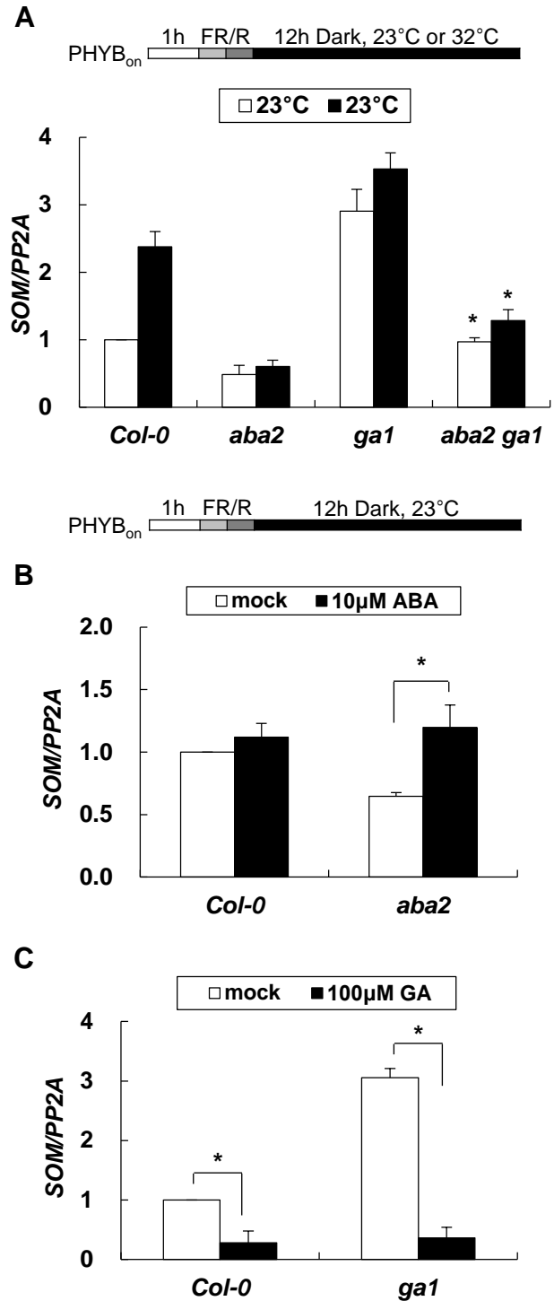
Supplemental Figure 2. Expression of SOM mRNA in the aba2 and the gal1 Mutant Seeds. (A) Relative SOM mRNA levels in Col-0, aba2 , gal1 , and aba2 gal1 double mutant seeds in response to high temperature. The top diagram indicates the light treatments and seed incubation conditions. The relative SOM mRNA level ( SOM/PP2A ) observed in Col-0 seeds incubated at 23°C was set to 1. Error bars indicate SD of three biological replicates (n = 3). The aba2 gal1 double mutant expressed slightly higher levels of SOM mRNA than the aba2 mutant at both 23°C and 32°C (*, p < 0.01, Student's t test). (B-C) Induction of SOM mRNA by ABA (10 μM) in the aba2 mutant seeds (B) and repression of SOM mRNA by GA (100 μM GA 4+7 ) in the gal1 mutant seeds (C) The relative SOM mRNA level ( SOM/PP2A ) of Col-0 seeds with mock treatment was set to 1 (SD, n = 3 biological replicates). * indicate statistical differences (p < 0.01, Student's t test).
