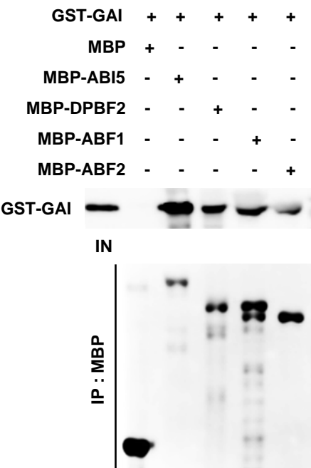
Supplemental Figure 8. In vitro co-precipitation assays between group A bZIPs and GAI. Amylose resins bound with MBP or MBP-fused group A bZIP (MBP-ABI5, -DPBF2, -ABF1, and -ABF2) proteins were incubated with GST-GAI proteins. IN represents 2% of the tested GST-GAI proteins. For immunoblotting assays, anti-GST (upper) or anti-MBP (lower) antibody was used.
