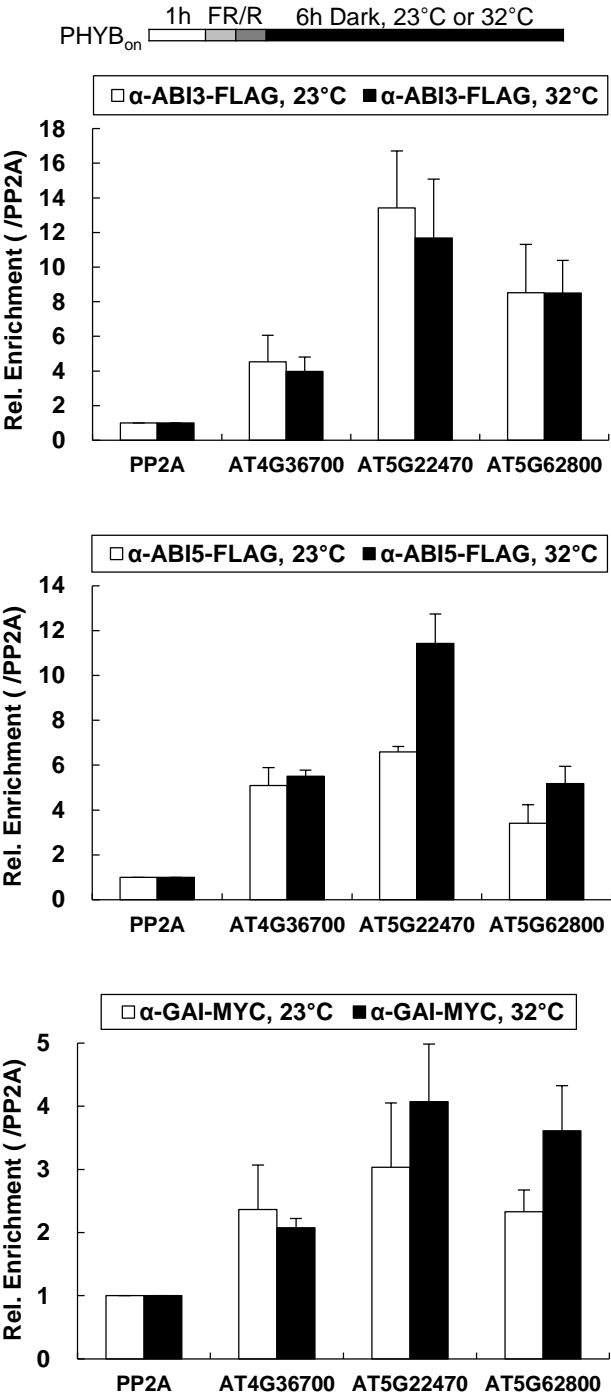
Supplemental Figure 7. ChIP assays were performed with anti-FLAG antibody in 35S:ABI3-FLAG ( \alpha -ABI3-FLAG) and 35S:ABI5-FLAG1 ( \alpha -ABI5-FLAG) transgenic seeds, or anti-MYC antibody in 35S:GAI-MYC ( \alpha -GAI-MYC) transgenic seeds incubated at 23°C or 32°C. The top diagram indicates the light treatments and seed incubation conditions. The co-precipitated level of each DNA fragment was quantified by real-time PCR and normalized with the input DNA level. The relative co-precipitated levels (IP DNA/input DNA) of PP2A were set to 1, and the relative enrichments of the other fragments compared to PP2A (/PP2A) are shown in the graph. Error bars indicate the SD of three biological replicates (n = 3).
