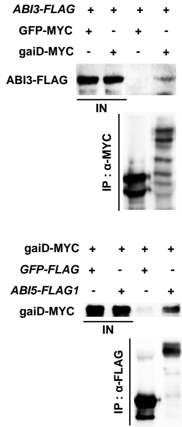
Supplemental Figure 5. In vivo co-precipitation assays between GAI and ABI3 (upper) or GAI and ABI5 (lower). 5-day-old, light-grown 35S:ABI3-FLAG , 35:GFP-FLAG , or 35:ABI5-FLAG1 transgenic seedlings were inoculated with Agrobacteria harboring 35S-driven GFP-MYC or gaiD-MYC vectors and incubated for 36 hours in the dark. Immunoprecipitation (IP) was performed with an anti-MYC (upper) or anti-FLAG antibody (lower). The input (IN) represents 1% of the tested seedling extracts. Co-precipitated ABI3-FLAG (upper) or gaiD -MYC (lower) were determined by immunoblotting assays using anti-FLAG or anti-MYC antibody, respectively.
