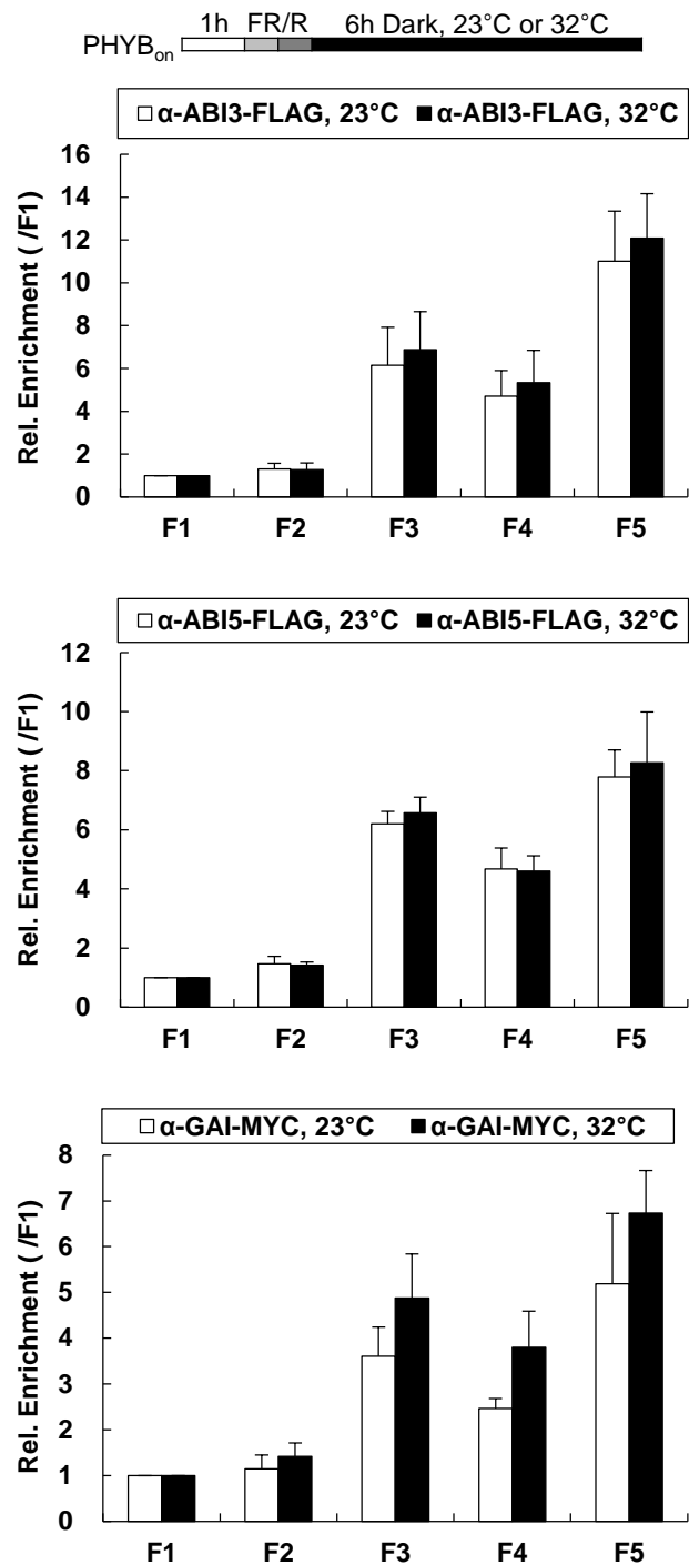
Supplemental Figure 4. ChIP assays were performed with anti-FLAG antibody in 35S:ABI3-FLAG ( \alpha -ABI3-FLAG) and 35S:ABI5-FLAG1 ( \alpha -ABI5-FLAG) transgenic seeds, or anti-MYC antibody in 35S:GAI-MYC ( \alpha -GAI-MYC) transgenic seeds incubated at 23°C or 32°C. The top diagram indicates the light treatments and seed incubation conditions. The co-precipitated level of each DNA fragment was quantified by real-time PCR and normalized with the input DNA level. The relative co-precipitated levels (IP DNA/input DNA) of F1 were set to 1, and the relative enrichments of the other fragments compared to F1 (/F1) are shown in the graph. Error bars indicate the SD of three biological replicates (n = 3).
