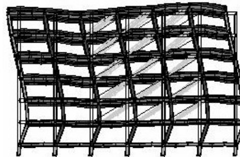
Fig.4.b.2 Mode shape 4 with 50% infill (frequency 4.807)
