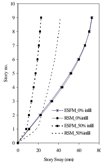
Fig. 9b. Story sway for 9 storied building for 50% infill and for no infill condition.
