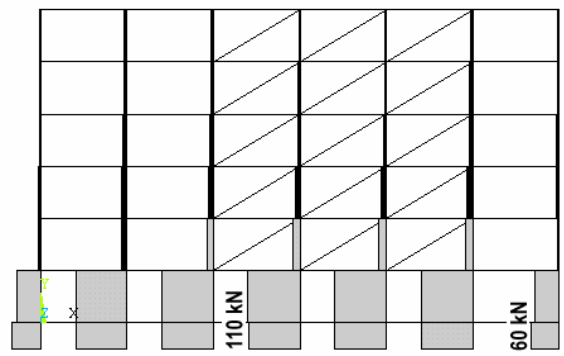
Fig. 6.b Distribution of shear force in columns due to response spectrum earthquake load for 50 percent infill condition.
