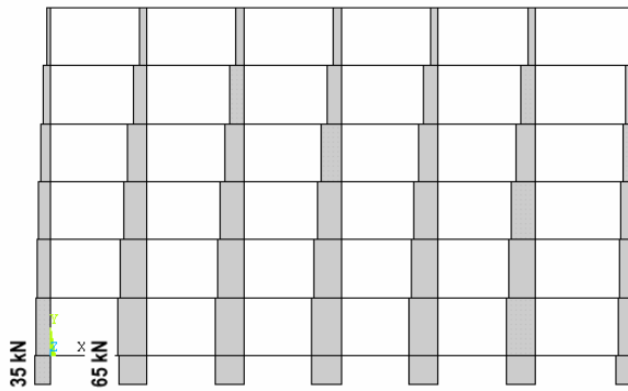
Fig. 6.a Distribution of shear force in columns due to response spectrum earthquake load for no infill condition .
