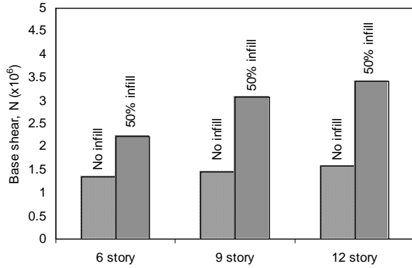
Fig.10 Comparison of base shear for different height of buildings.
