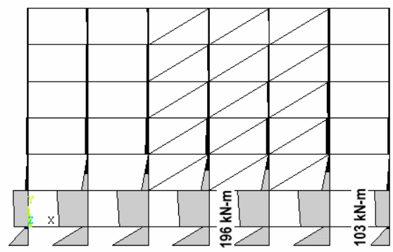
Fig. 7.b Distribution of bending moment in columns due to response spectrum earthquake load for 50 percent infill condition.
