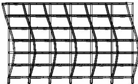
Fig.4.b.1 Mode shape 4 without infill (frequency 2.336)
