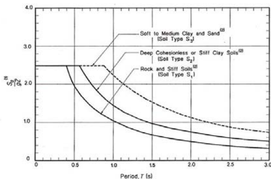
Fig.3 Normalized Response Spectra for 5% Damping Ratio [8].
