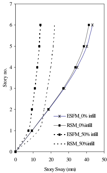
Fig. 9a. Story sway for 6 storied building for 50% infill and for no infill condition.
