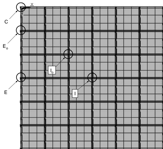
Fig.2.a FE mesh of the building in plan.
