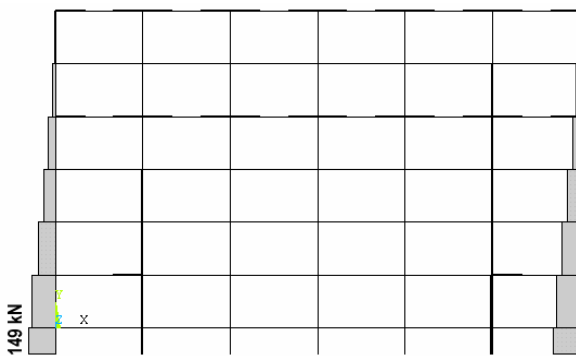
Fig. 8.a Distribution of axial force in columns due to response spectrum earthquake load for no infill condition.
