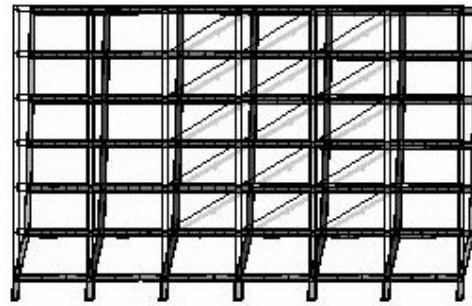
Fig.4.a.2 Mode shape 1 with 50% infill (frequency 1.278)
