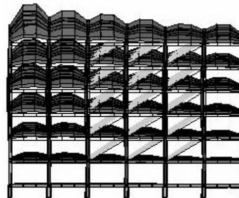
Fig.4.c.2 Mode shape 7 with 50% infill (frequency 7.438)
