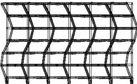
Fig.4.c.1 Mode shape 7 without infill (frequency 4.104)
