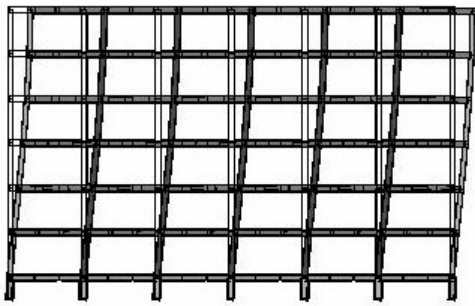
Fig.4.a.1 Mode shape 1 without infill (frequency 0.755)
