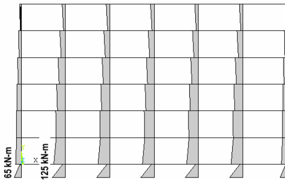
Fig. 7.a Distribution of bending moment in columns due to response spectrum earthquake load for no infill condition.
