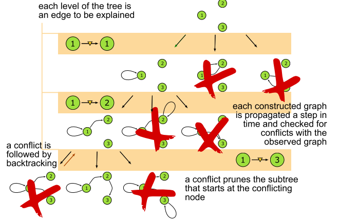
Figure 2: The search tree for 3-node SCC of Figure 1
