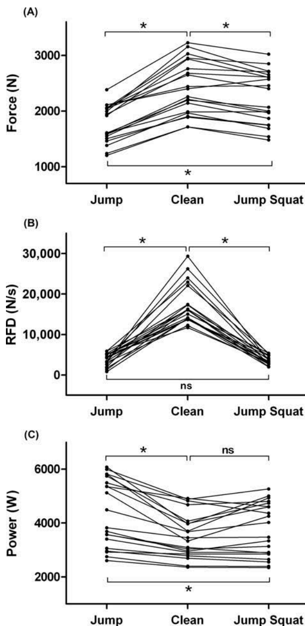
Figure 2. (A) Peak vertical ground reaction force, (B) peak rate of force development (RFD), and (C) peak power generated during the upward phase of the jump, power clean and jump squat. Connected dots indicated individual participants. (* indicates P \leq .05 ; ns = not significant)
