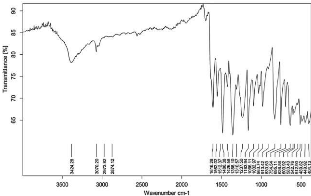
IR spectrum of complex [\{Co(HL)\}_2]
