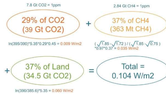
Fig 4.4b: Detailed calculations on the annual change in radiative forcing if the Killing machine is shut down, including CO 2 , Methane and Land Use changes, while neglecting the impact of other minor greenhouse gases.
