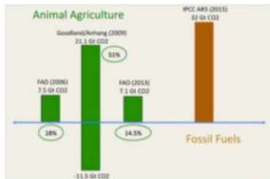
Fig. 4.4. Lifecycle emissions of Animal Agriculture as measured by the UN FAO (two versions) and World Bank scientists, Goodland and Anhang, in comparison with the total CO 2 emissions from fossil fuel sources.
