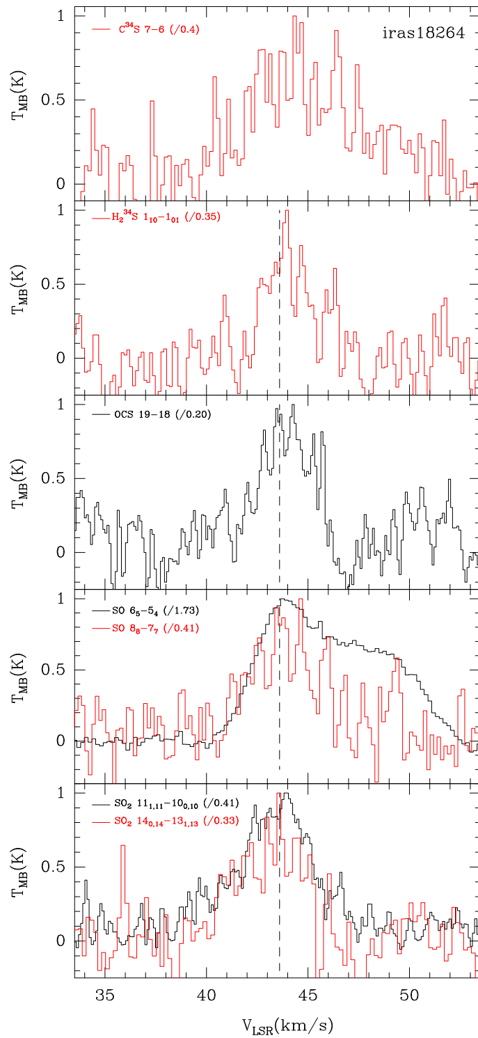
Fig. 15. Normalized emission of CS, H 2 S, OCS, SO, SO 2 (and isotopic species) lines from IRAS18264–1152. Spectra velocity resolutions are 0.10-0.19 km s -1 . The dashed line shows the source LSR velocity.
