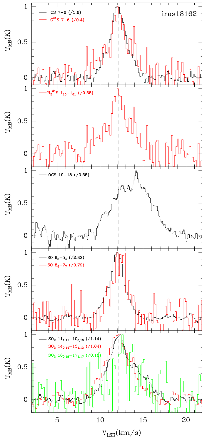
Fig. 17. Normalized emission of CS, H 2 S, OCS, SO, SO 2 (and isotopic species) lines from IRAS18162–2048. Spectra velocity resolutions are 0.10-0.19 km s -1 . The dashed line shows the source LSR velocity.
