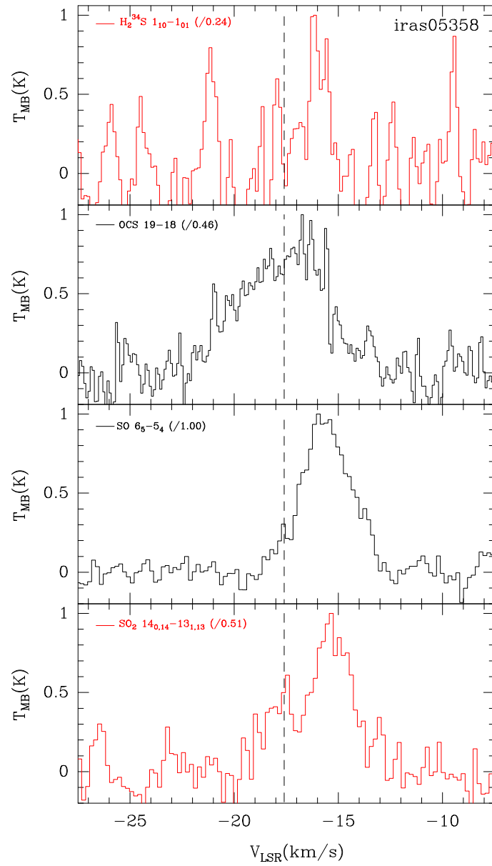
Fig. 16. Normalized emission of CS, H 2 S, OCS, SO, SO 2 (and isotopic species) lines from IRAS05358+3543. Spectra velocity resolutions are 0.10-0.19 \text{km s}^{-1} . The dashed line shows the source LSR velocity.
