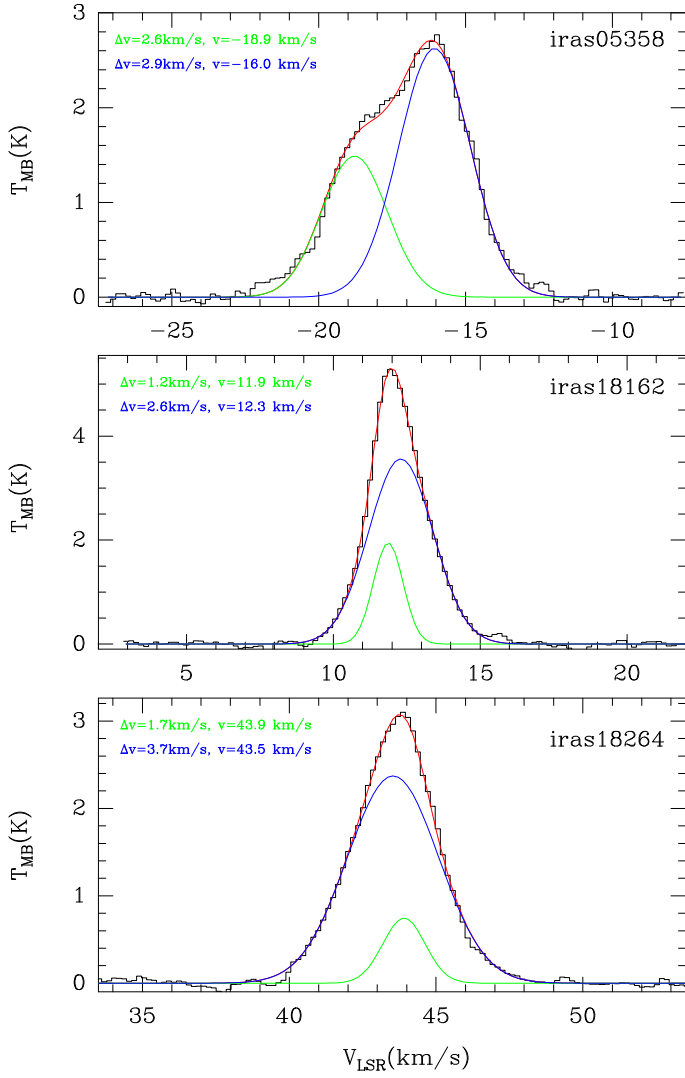
Fig. 6. Gaussian fit of the SO 3_4 - 2_3 line emission from IRAS05358+3543, IRAS18162–2048 and IRAS18264–1152. The observed spectra are in black, total fit in red, individual components in blue and green.
