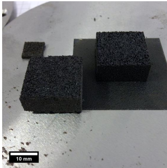
Figure 5 – Various geometrical shapes manufactured using an energy density of 1.011 J/mm 2 .
