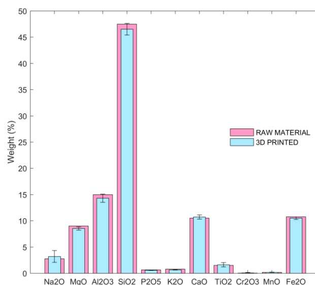
Figure 9 – Elemental concentrations % between processed (3D PRINTED) and un-processed (RAW MATERIAL) regolith simulant acquired via \mu XRF.
